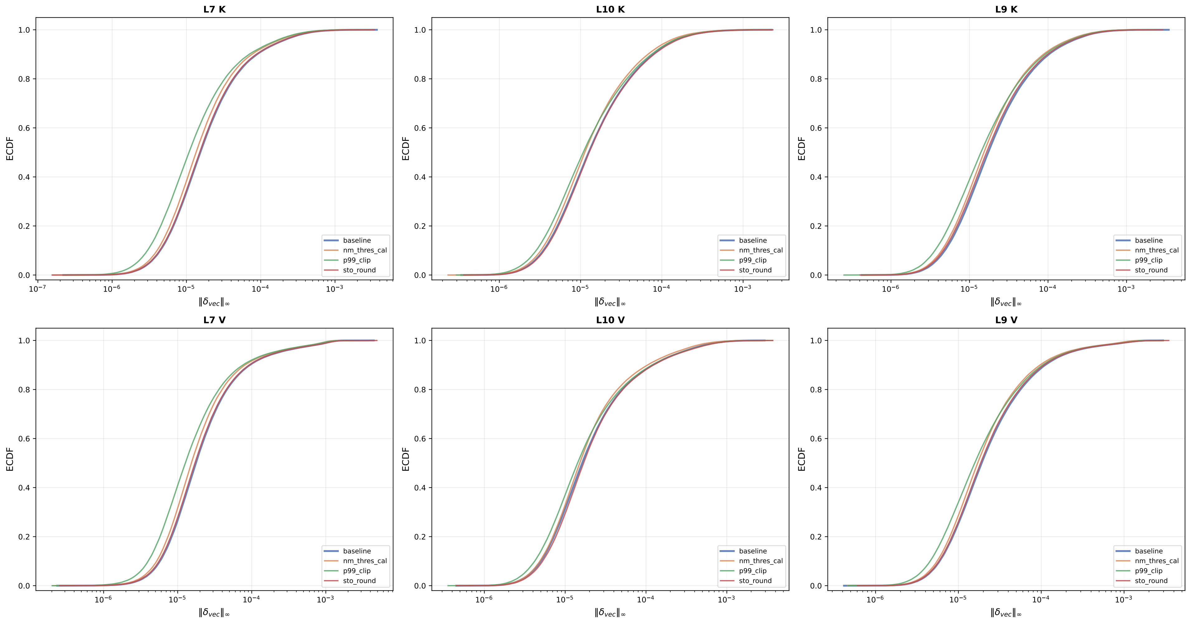
Absmax ECDF — Solution Comparison (DAC 7-bit) Do solutions change the gradient magnitude distribution? (Note: absmax distribution \neq quantization underflow; see QZR heatmap for that)
