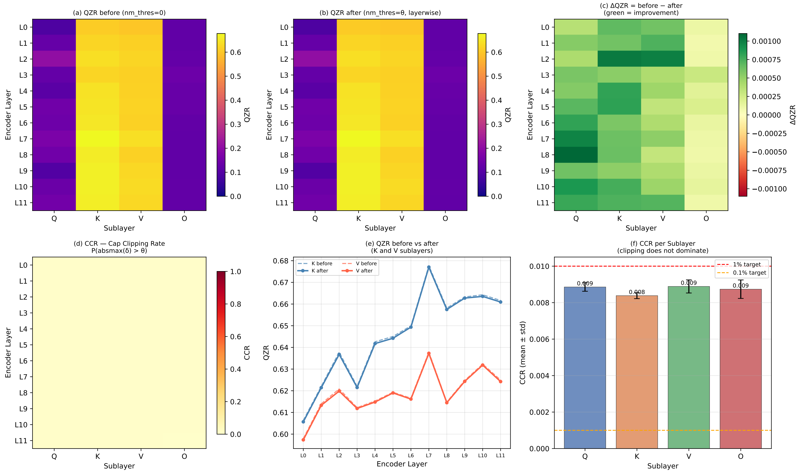
Figure 2 — nm_thres Calibration Effect: BERT-base Q/K/V/O Analog Tiles (mode=layerwise, q=0.99, safety=1.1, DAC=7-bit, N=200 steps) \theta_{lw}=[0.00001, 0.00083]
