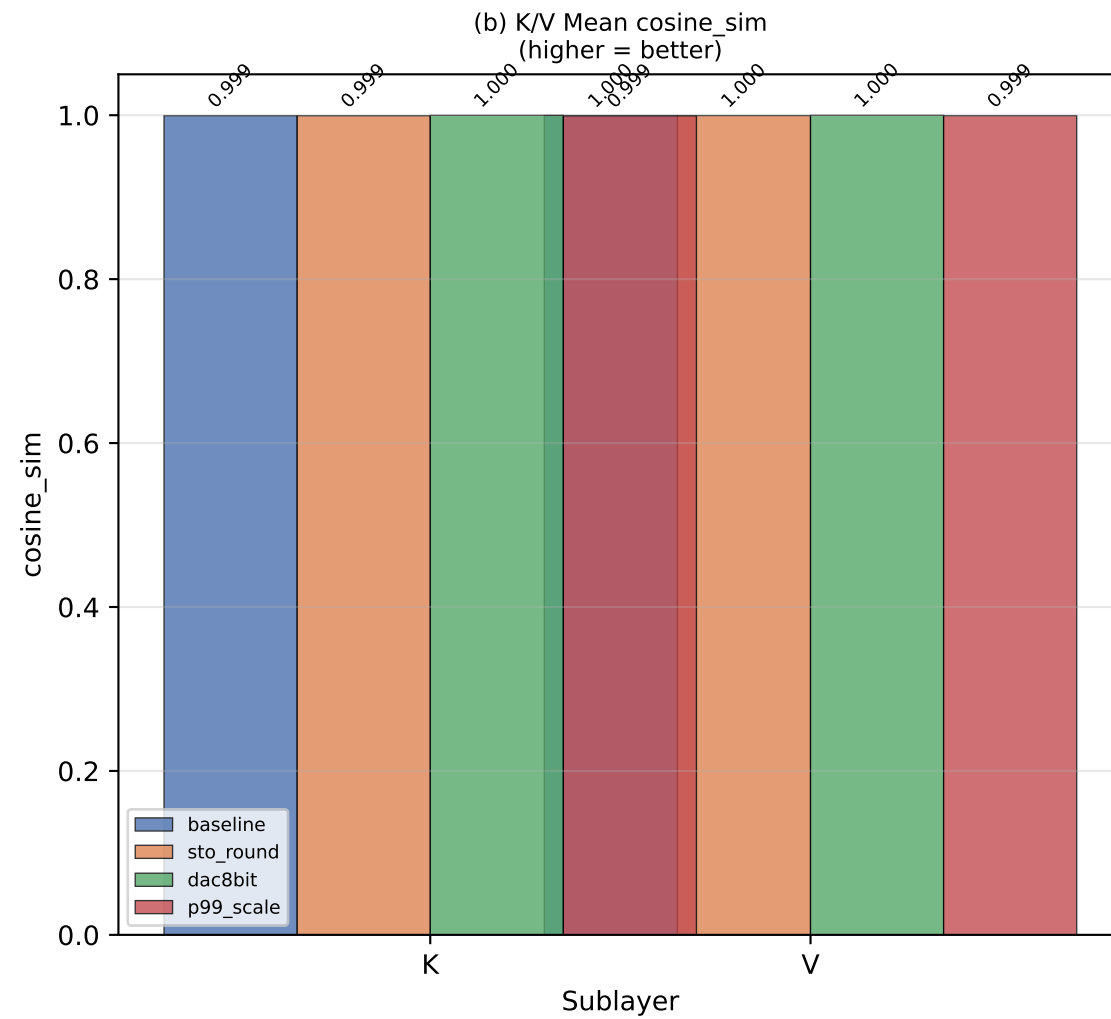
Figure 3 — Alternative Solution Comparison (K/V sublayers) BERT-base, 200 steps × batch 8
