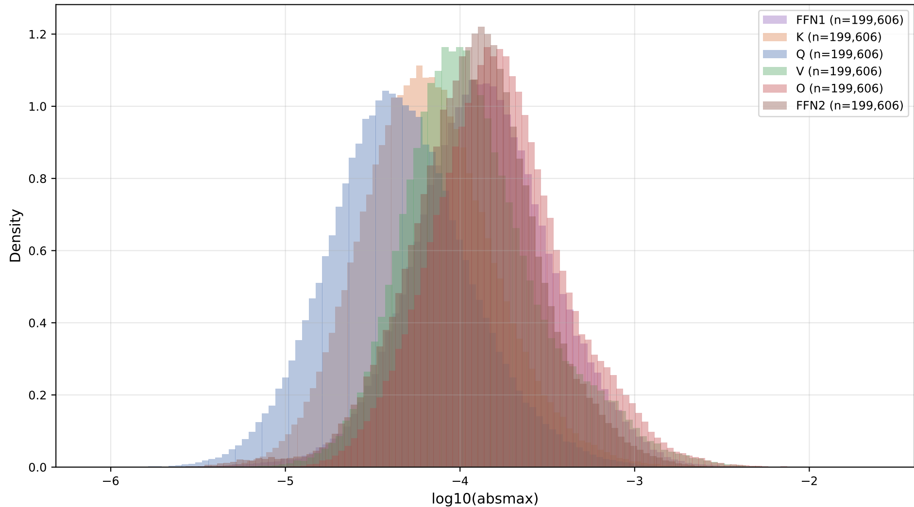
CoLA — Absmax Distribution by Sublayer (L0-10 pooled)
