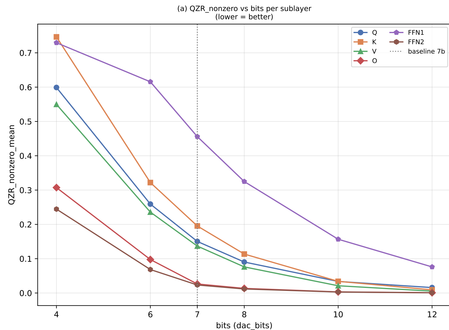
Figure B — IO Resolution Sweep (BERT-base, bits=[np.int64(4), np.int64(6), np.int64(7), np.int64(8), np.int64(10), np.int64(12)]) sweep: dac_bits=adc_bits=bits, 3 steps; baseline: dac=7b, adc=9b, 5 steps
