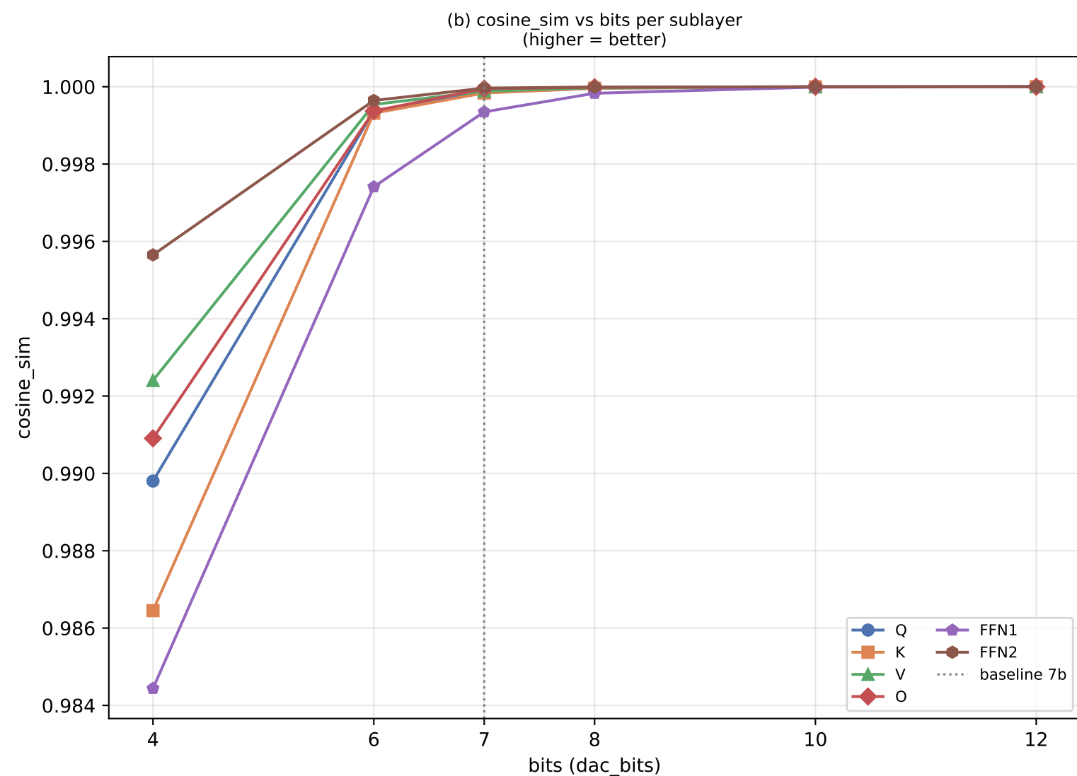
Figure B — IO Resolution Sweep (BERT-base, bits=[np.int64(4), np.int64(6), np.int64(7), np.int64(8), np.int64(10), np.int64(12)]) sweep: dac_bits=adc_bits=bits, 3 steps; baseline: dac=7b, adc=9b, 5 steps
