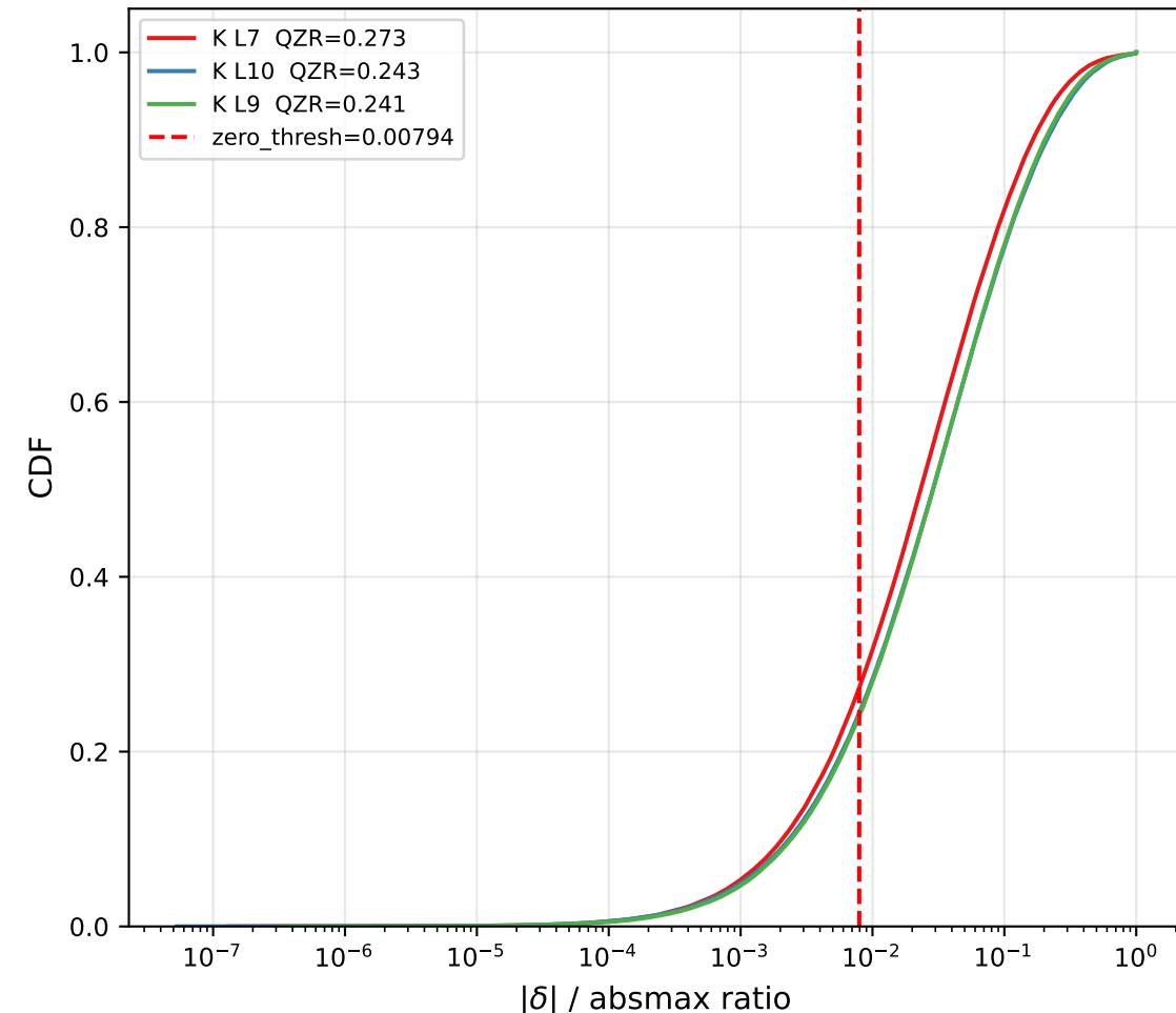
(c) CDF of gradient ratio — worst K layers
