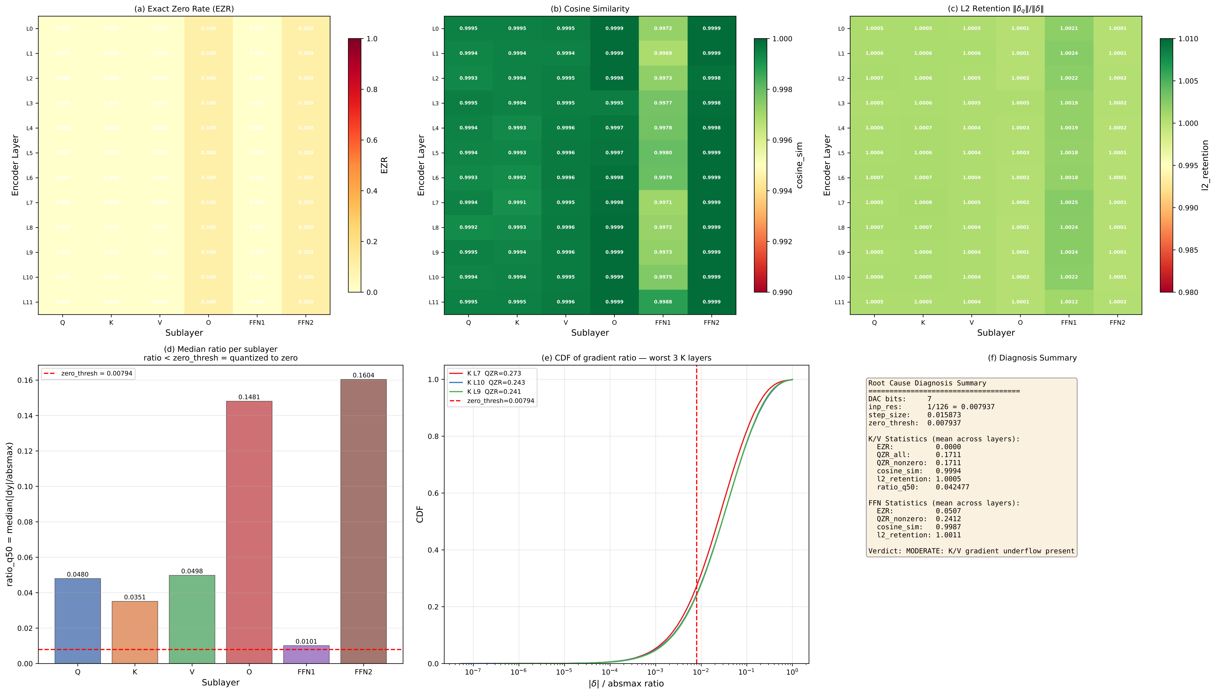
Supplementary Figure S1 — Root Cause Diagnosis Detail (BERT-base, DAC=7-bit, 6 sublayers)
