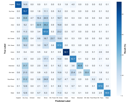
Figure 13: Row-normalized confusion matrix for DACS on the L2 task. Rural Road recall drops to 8.2%, with 24.8% misclassified as Shrub Forest and 31.2% as Dry Cropland under domain shift.
