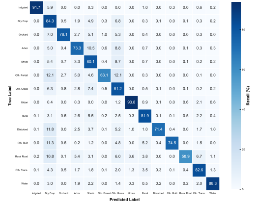
Figure 12: Row-normalized confusion matrix for SETR on the L2 task. Rural Road shows 58.9% correct classification, with 3.1% misclassified as Shrub Forest and 10.8% as Dry Cropland.
