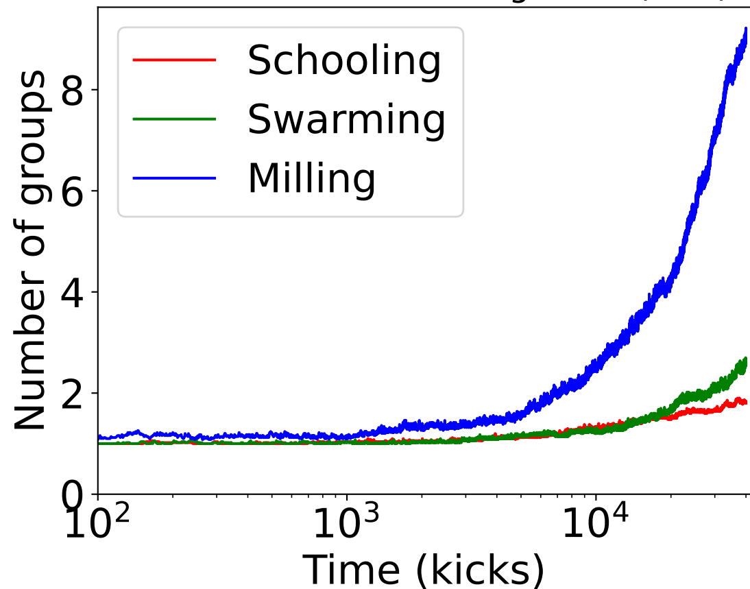
Number of groups through time for three different emergences ( k=1 )
