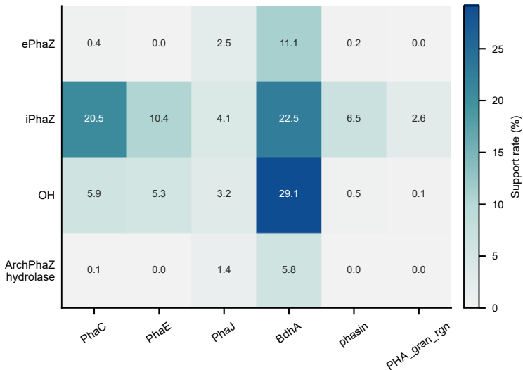
Core candidate families
