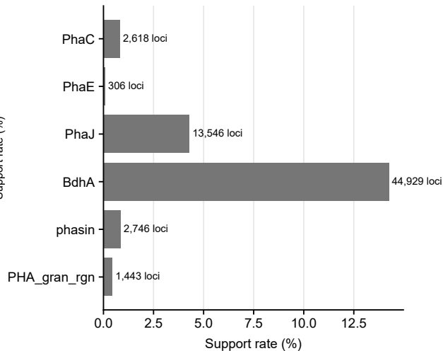
ArchPhaZ patatin candidates
