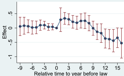
TWFE estimates
