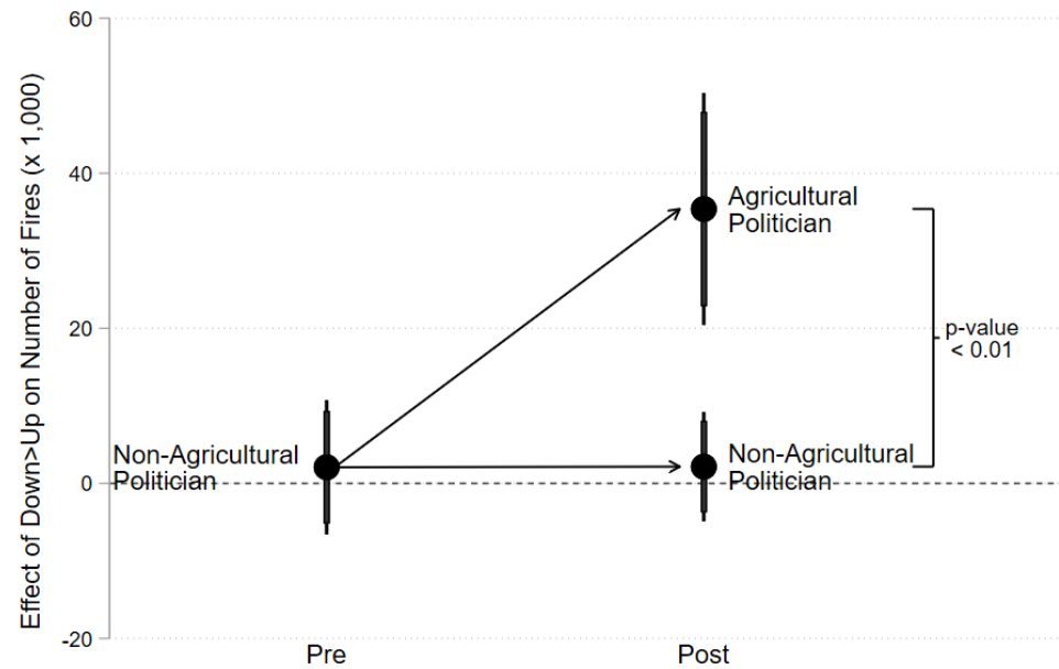
DiD interaction: \text{post} \times \text{treat} \times \text{downup\_ac\_pop}
