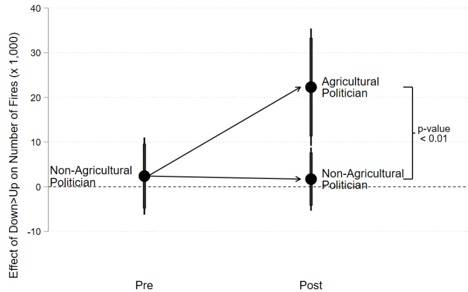
DiD interaction: post \times treat \times downup_ac_pop
