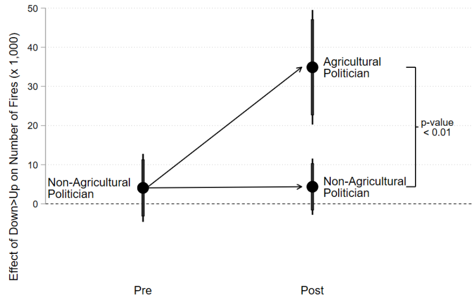
DiD interaction: \text{post} \times \text{treat} \times \text{downup\_ac\_pop}
