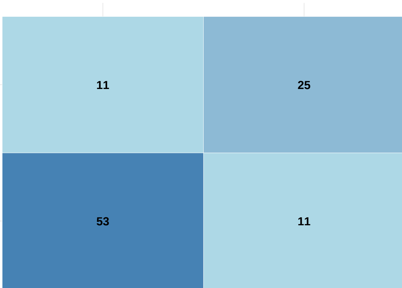
Confusion Matrix
