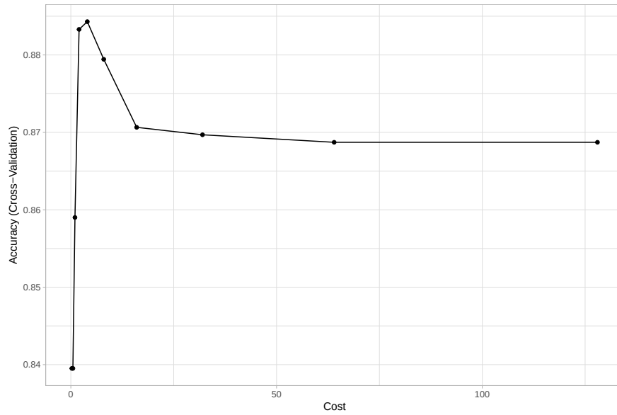
Figure 1: Plotting the results, we see that smaller values of the cost parameter ( C \approx 2-8 ) provide better cross-validated accuracy scores for these training data.
