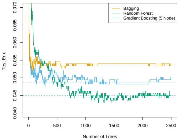
Spam Data
