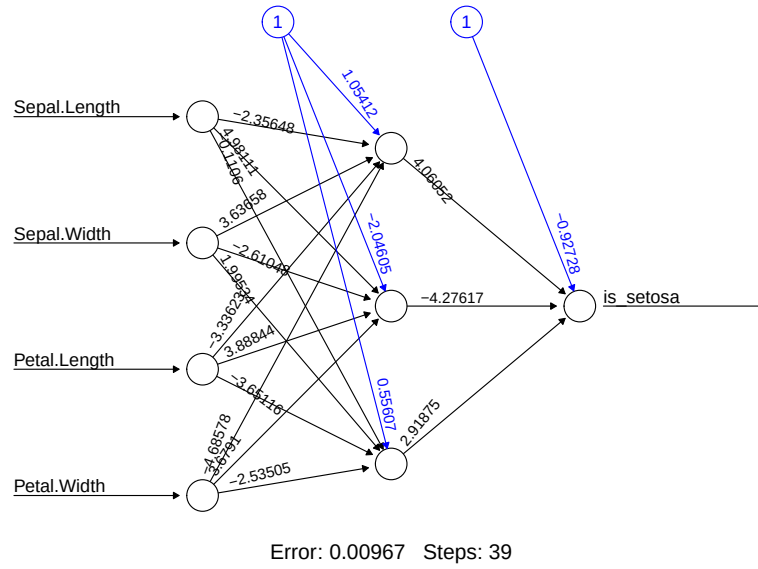
Figure 1: This diagram illustrates a feed-forward ANN with four input nodes, a single three-unit hidden layer, and a binary output for setosa identification. It visualizes the specific connection weights and bias values refined through training to achieve minimal prediction error.
