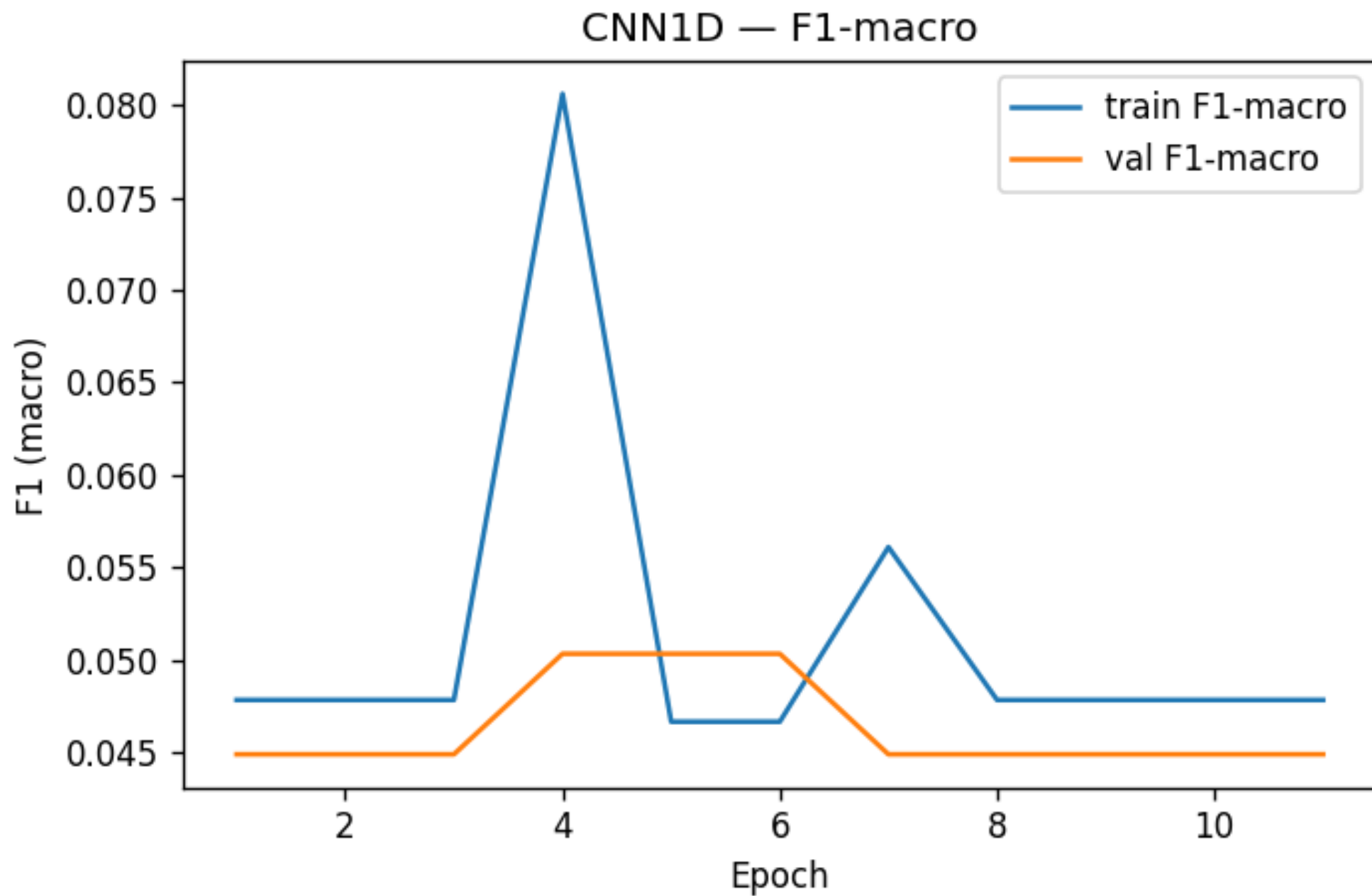
Figure 014: figures/curves/cnn1d_f1.png
