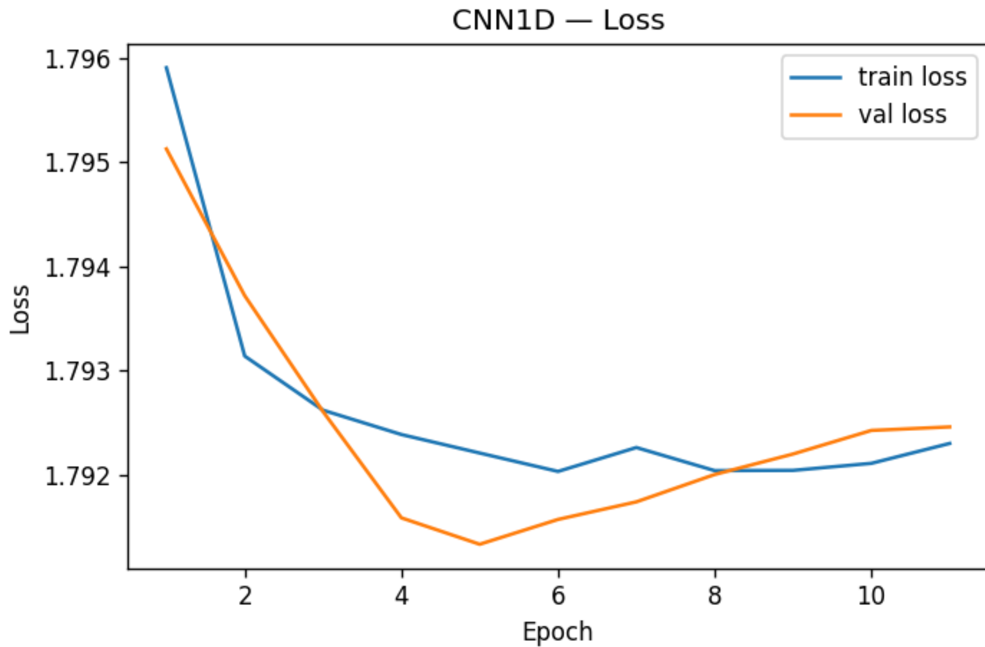
Figure 018: figures/curves/cnn1d_loss_replot.png
