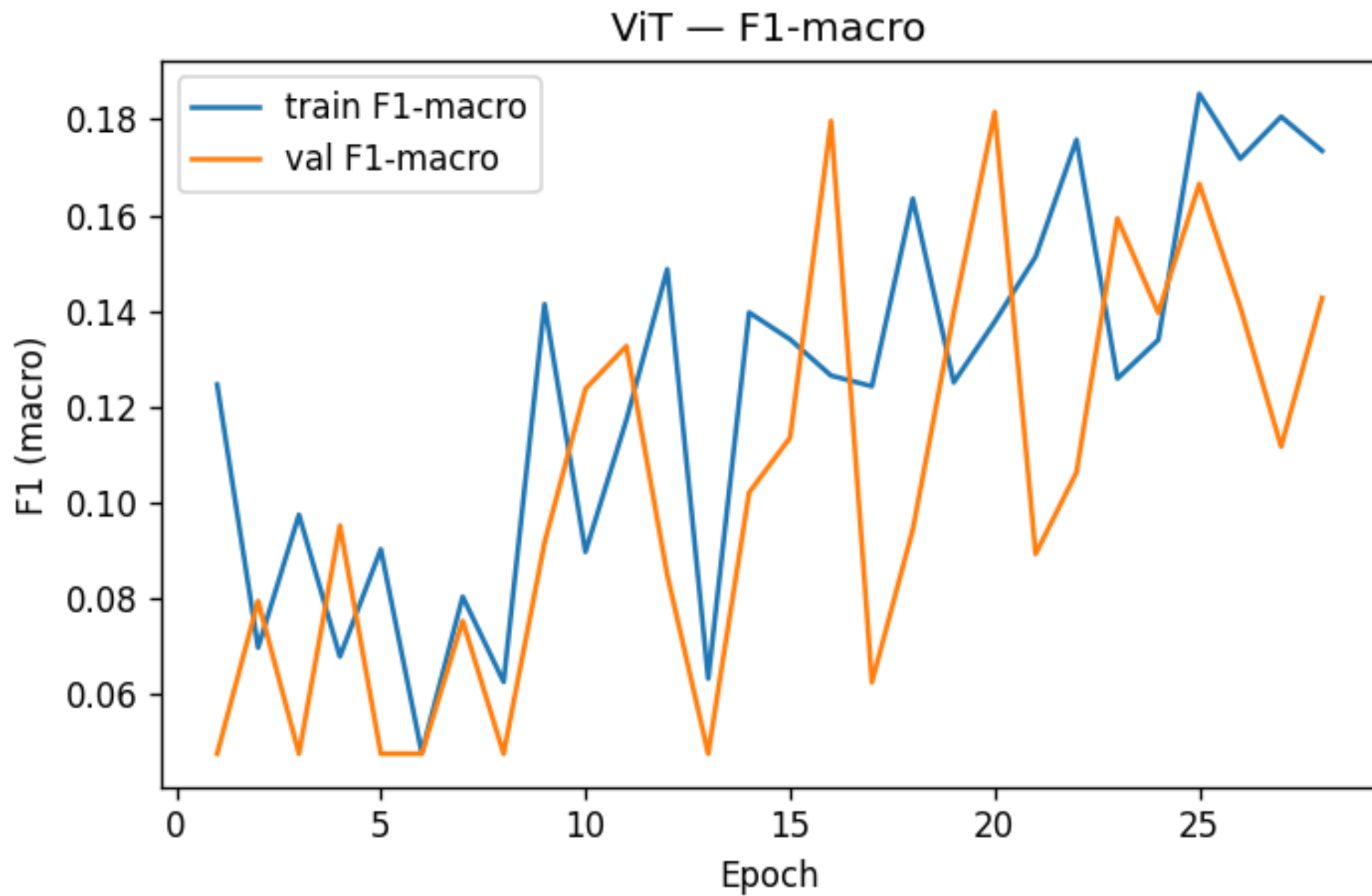
Figure 022: figures/curves/vit_f1.png
