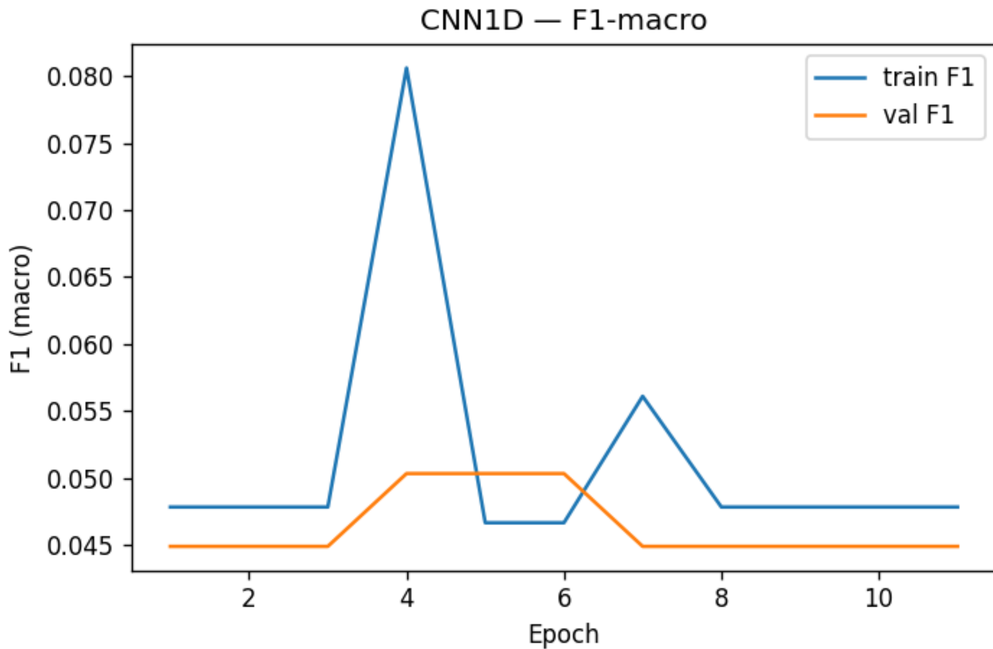
Figure 015: figures/curves/cnn1d_f1_replot.png
