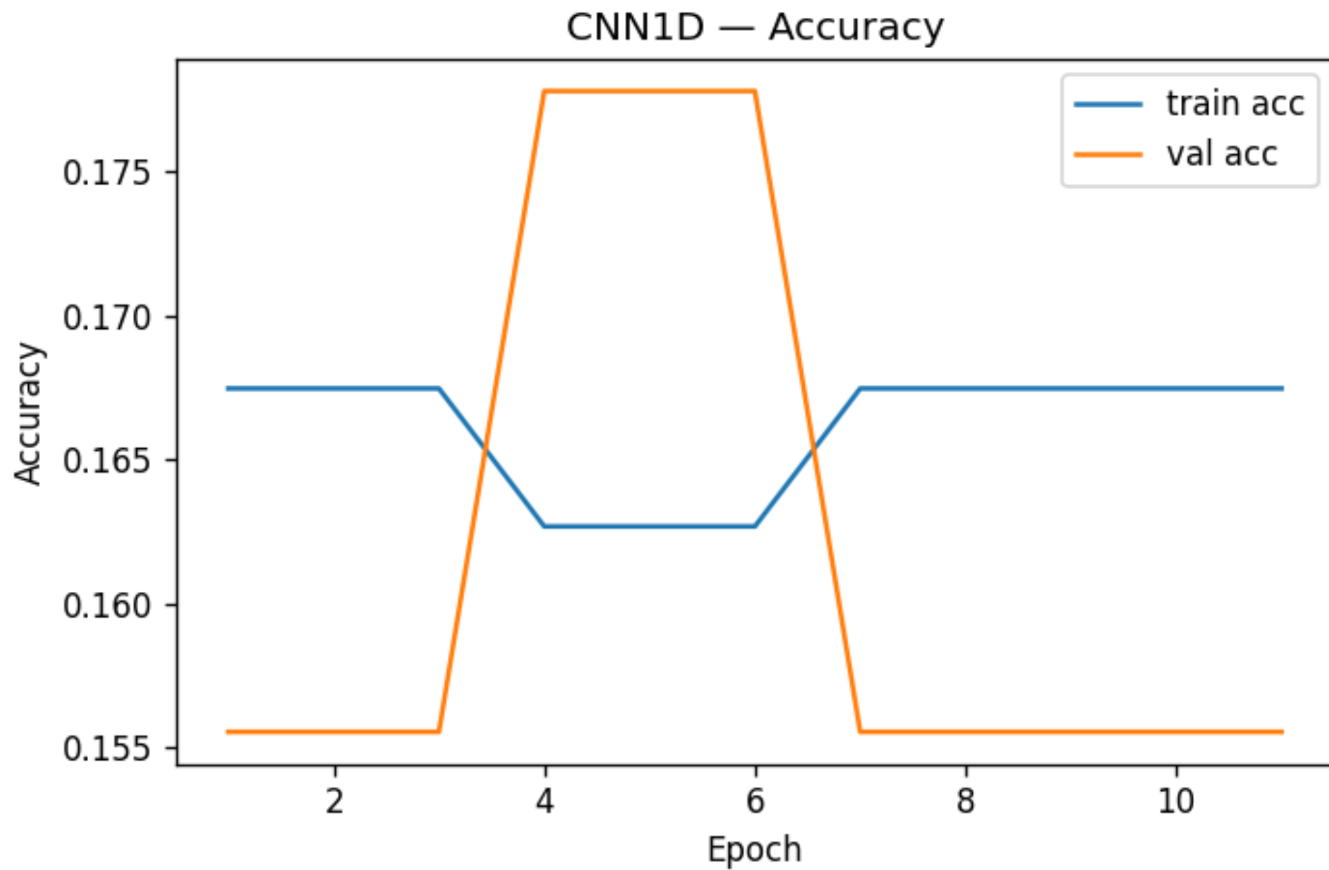
Figure 013: figures/curves/cnn1d_acc_replot.png
