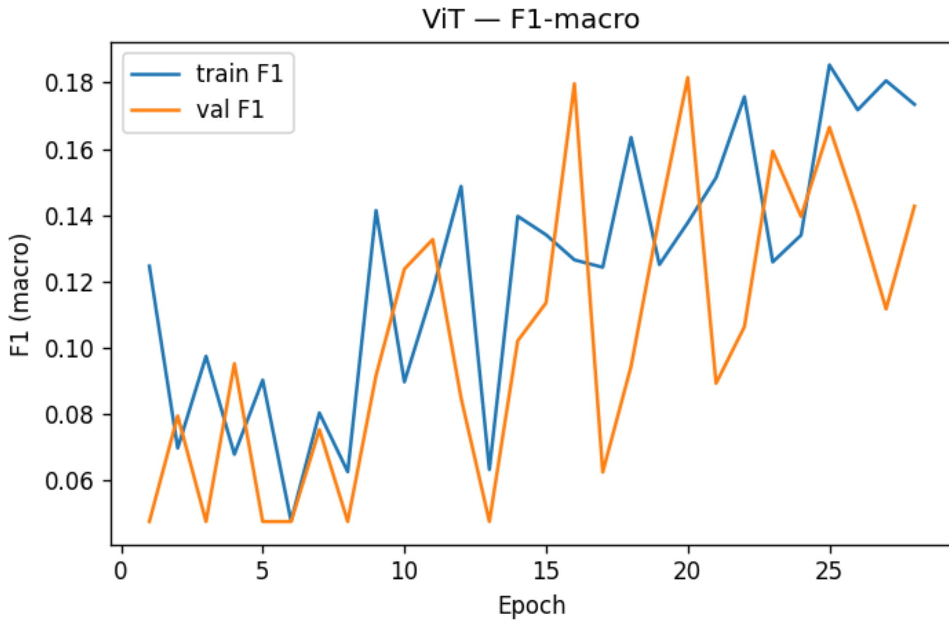
Figure 023: figures/curves/vit_f1_replot.png
