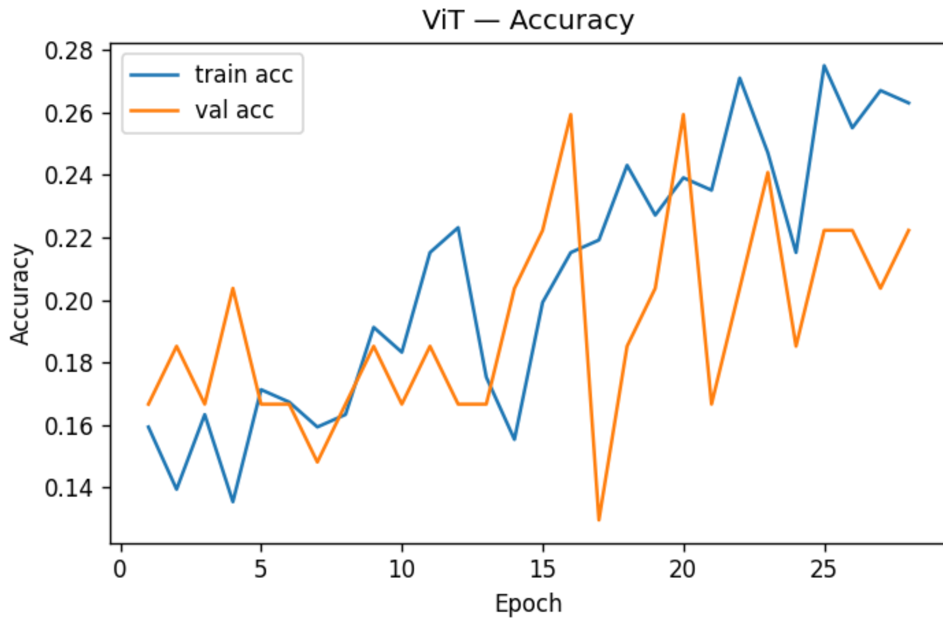
Figure 020: figures/curves/vit_acc.png
