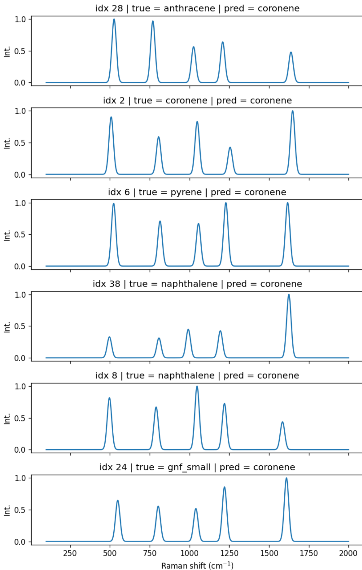
Figure 016: figures/curves/cnn1d_inference_examples.png
