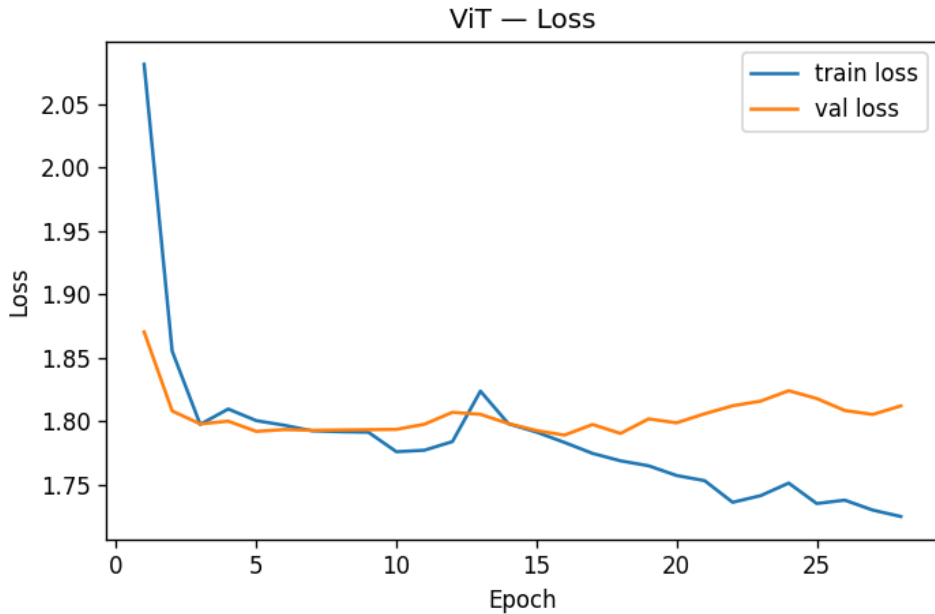
Figure 024: figures/curves/vit_loss.png
