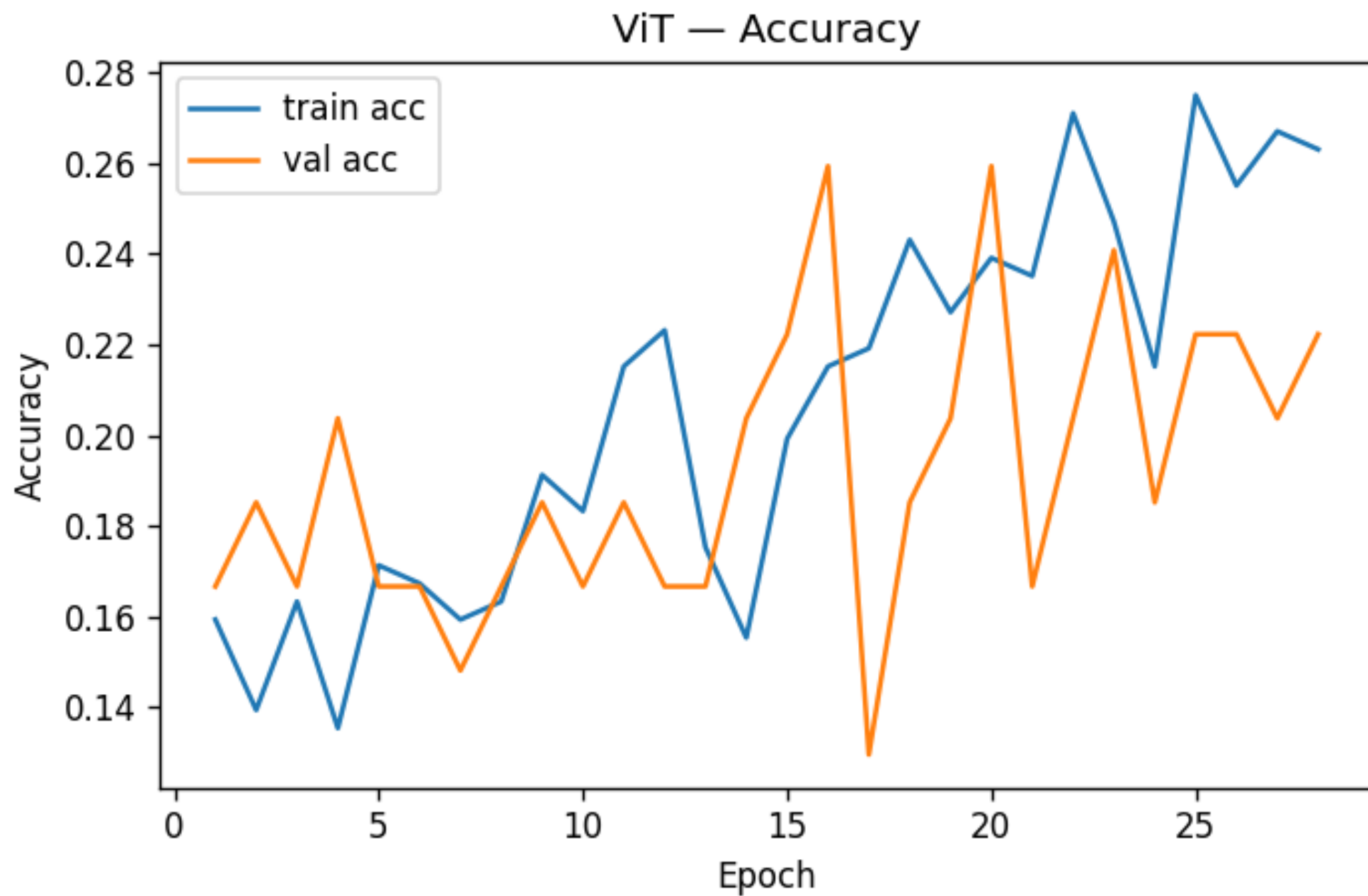
Figure 021: figures/curves/vit_acc_replot.png
