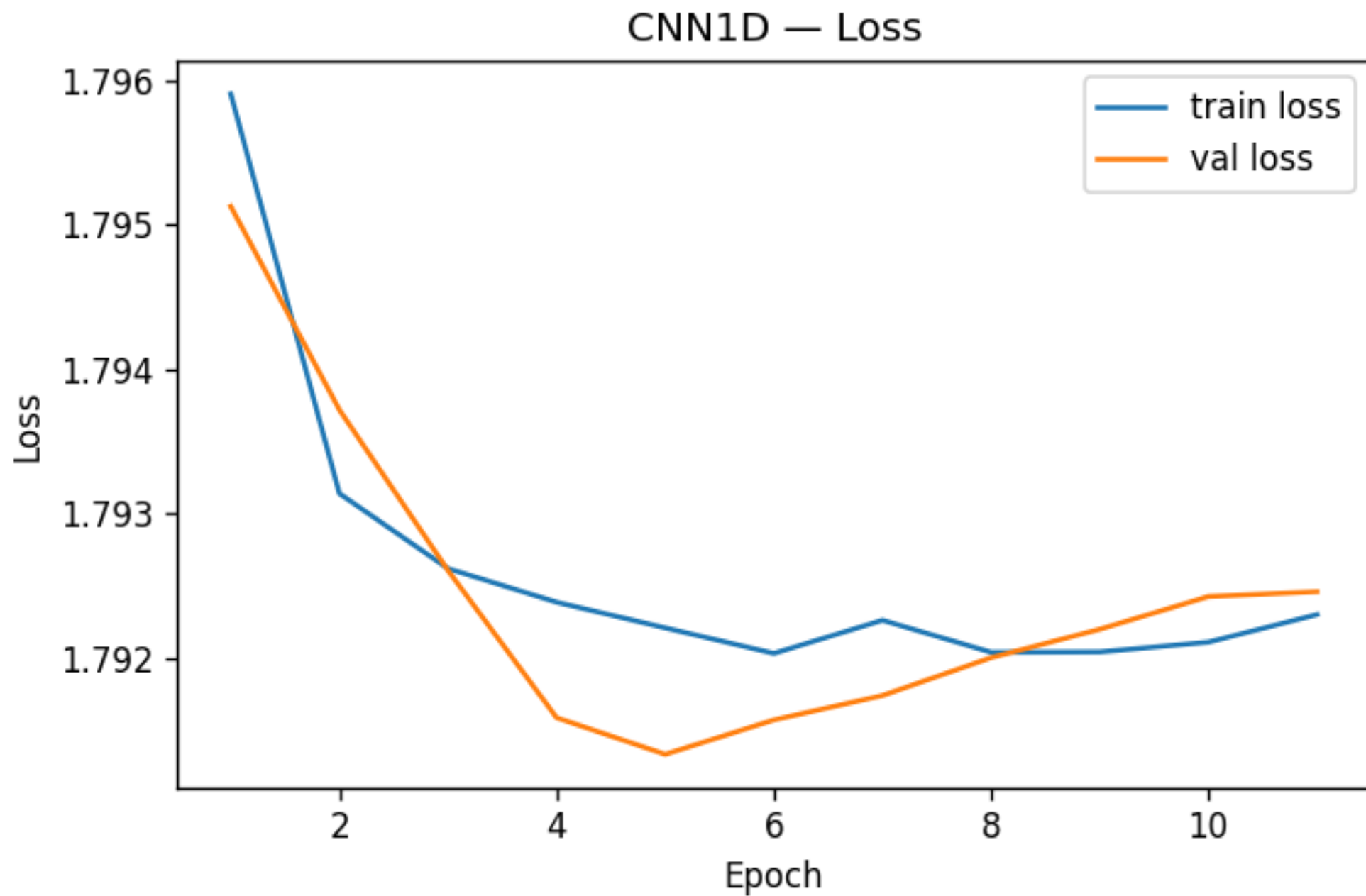
Figure 017: figures/curves/cnn1d_loss.png
