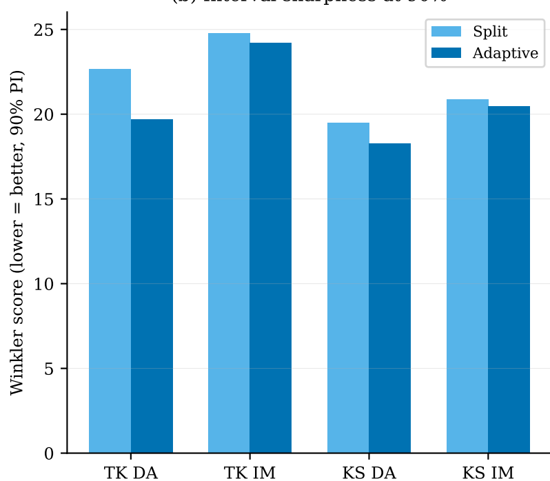
(b) Interval sharpness at 90%
