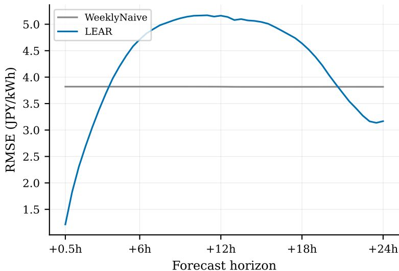
KS DA (rRMSE=0.987)
