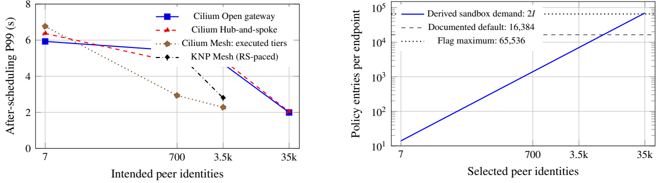
Figure 2: Different meanings of scaling. Left: measured per-run startup quantiles for ReplicaSet-paced tiers (connecting lines are visual guides; KNP Tier 1 5,000-ppr burst at 151.5 s and Tier 4 unbuffered raw-Pod queue drain at 421.4 s are omitted from the 0–8 s vertical scale). Right: conditional permission-state model for eager per-endpoint compilation. In agentic-cilium.k8s.local, -bpf-policy-map-max was raised to 65,536, permitting unidirectional 35k tiers while excluding bidirectional mesh at 35k ( 2I = 70,000 > 65,536 ).
