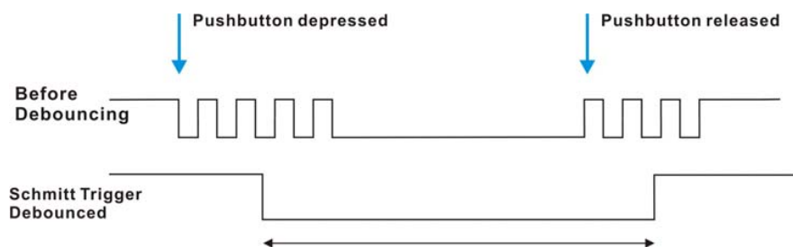
Figure 4.3. Switch debouncing.
