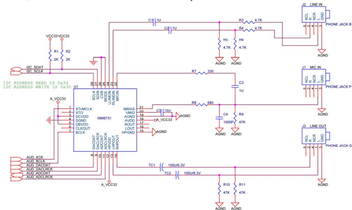
Figure 4.15. Audio CODEC schematic.
