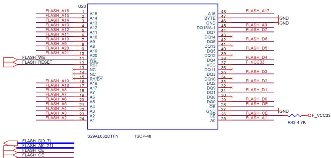
Figure 4.25. Flash schematic.
