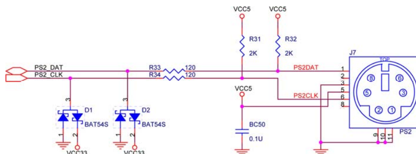
Figure 4.17. PS/2 schematic.
