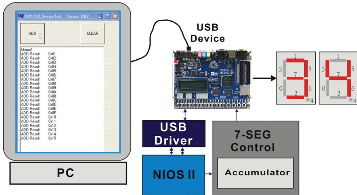
Figure 5.6. The setup for the USB device demonstration.
