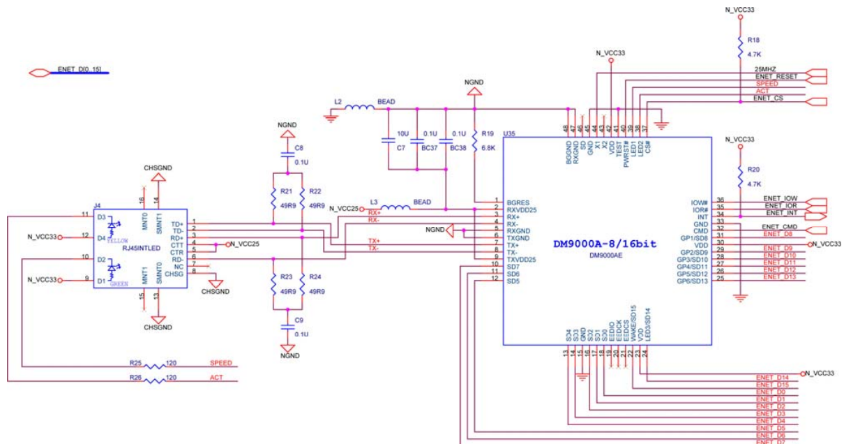
Figure 4.18. Fast Ethernet schematic.
