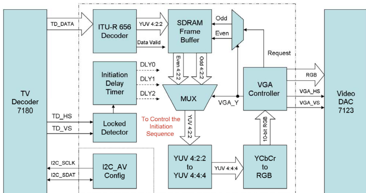
Figure 5.1. Block diagram of the TV box demonstration.
