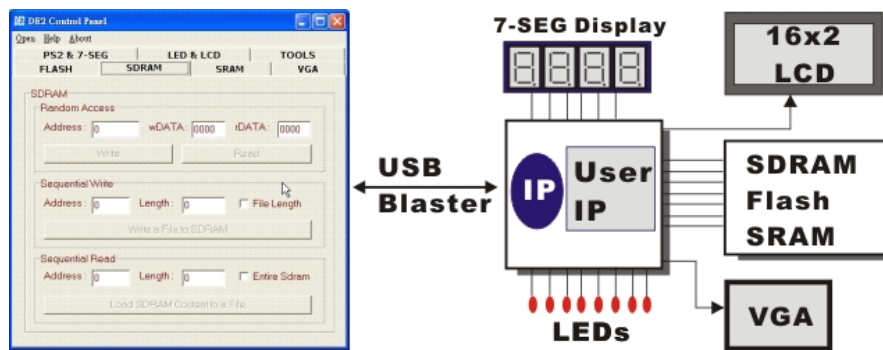
Figure 3.3. The DE2 Control Panel concept.
