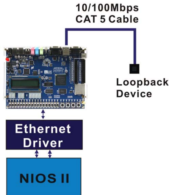
Figure 5.10. The setup for the Ethernet demonstration.
