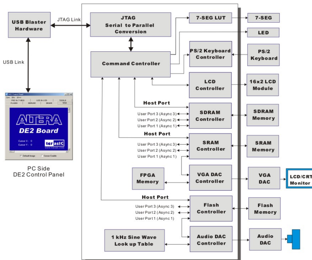
Figure 3.7. The DE2 Control Panel block diagram.
