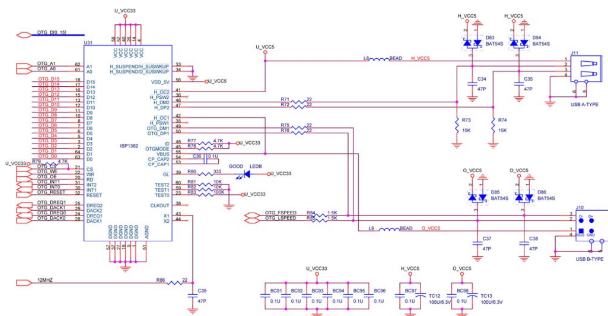
Figure 4.21. USB (ISP1362) host and device schematic.
