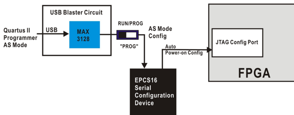
Figure 4.2. The AS configuration scheme.
