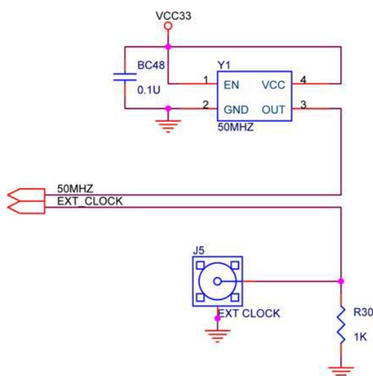
Figure 4.8. Schematic diagram of the clock circuit.
