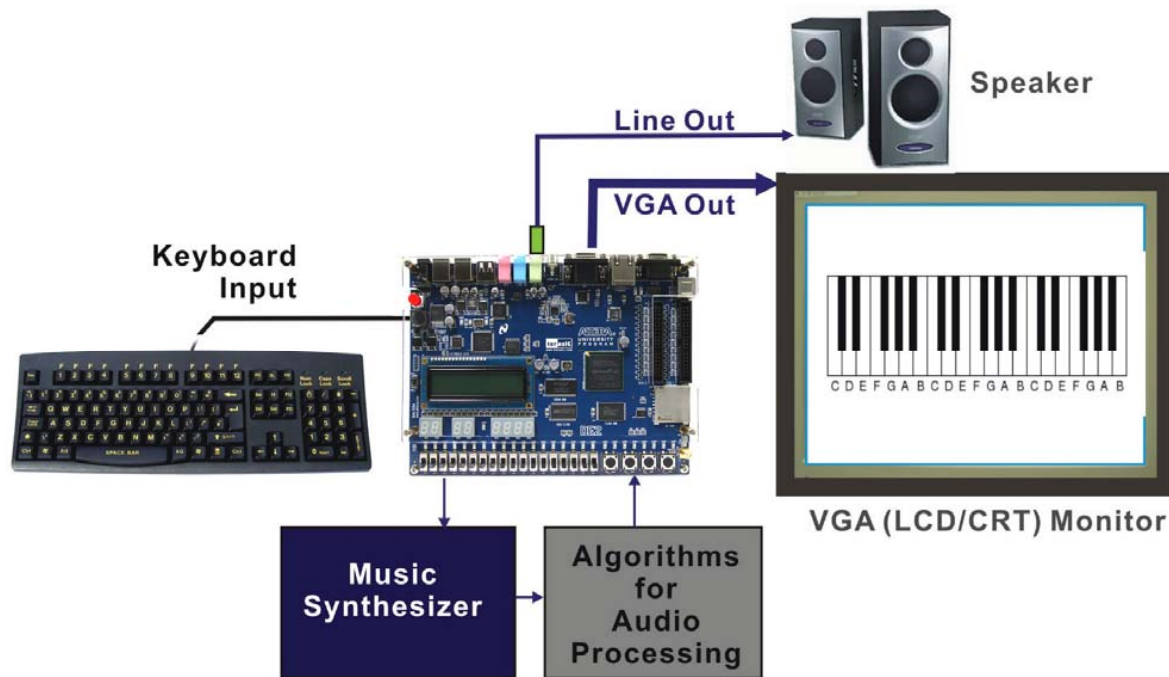
Figure 5.14. The Setup of the Music Synthesizer Demonstration.
