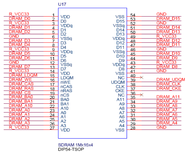
Figure 4.23. SDRAM schematic.
