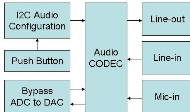
Figure 5.7. Block diagram of the Karaoke Machine demonstration.
