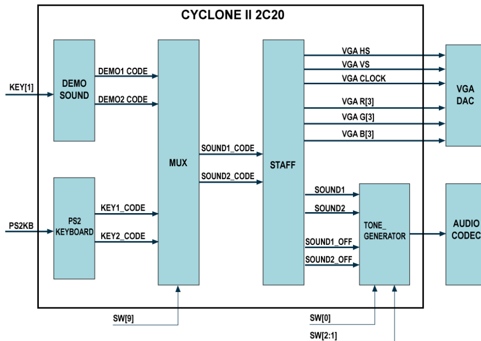
Figure 5.13. Block diagram of the Music Synthesizer design
