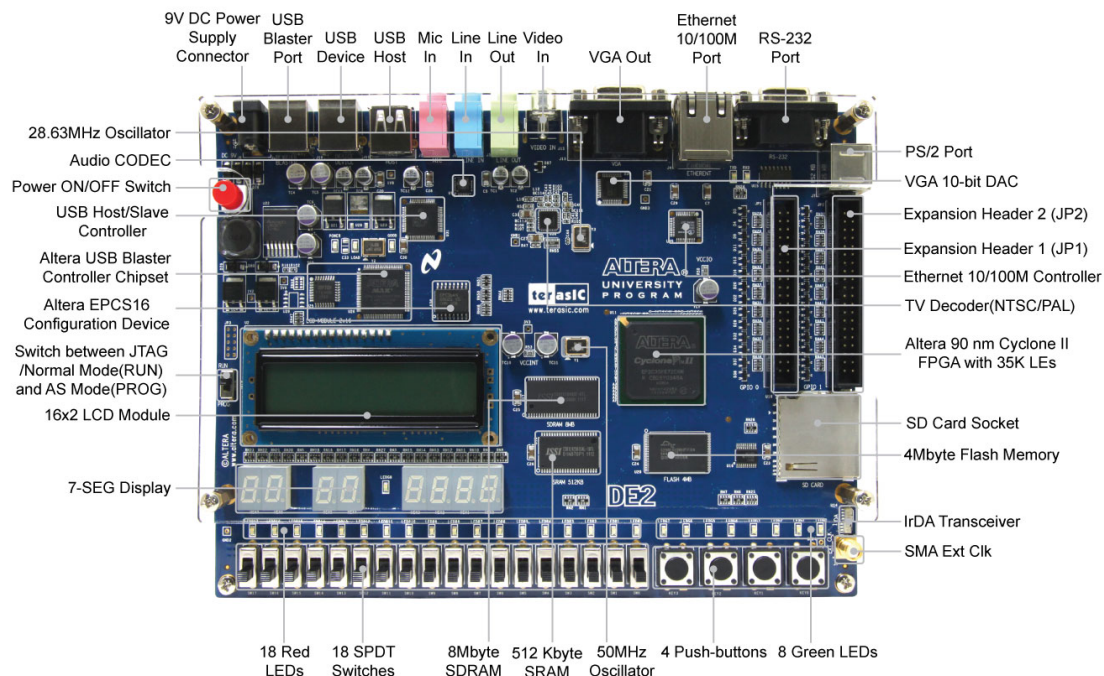
Figure 2.1. The DE2 board.
