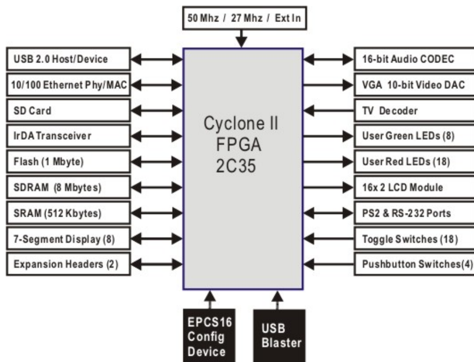
Figure 2.2. Block diagram of the DE2 board.
