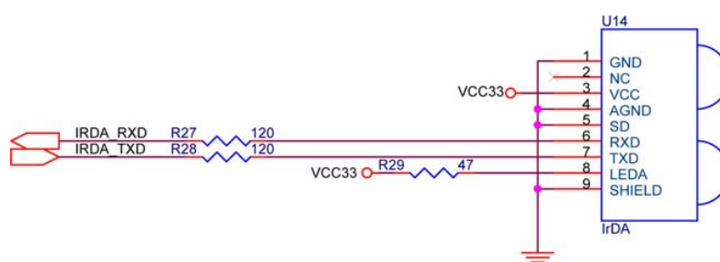
Figure 4.22. IrDA schematic.
