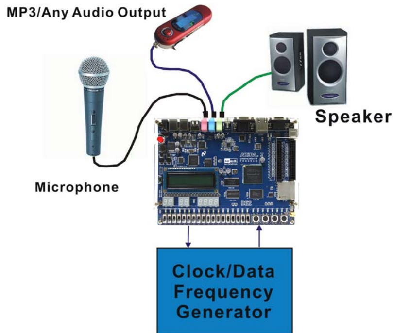
Figure 5.8. The setup for the Karaoke Machine.
