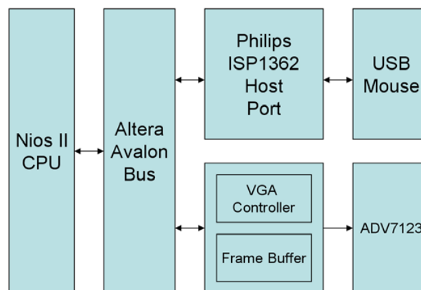
Figure 5.3. Block diagram of the USB paintbrush demonstration.
