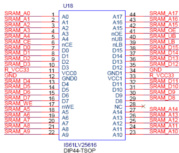
Figure 4.24. SRAM schematic.
