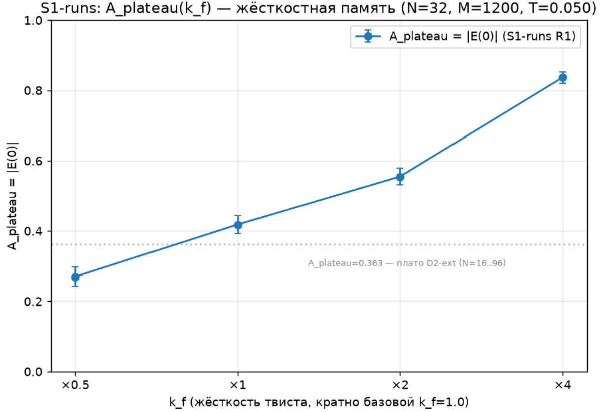
Fig. 2. A_{\text{plateau}}(k_f) — stiffness memory. Four points with 1\sigma error bars from the frozen S1-runs R1 raw data ( N = 32 , M = 1200 , T = 0.05 ; commit a9cef7b). Dotted line: the D2-ext plateau A_{\text{plateau}} = 0.363 of Section 6.1, measured over N \in [16, 96] .
