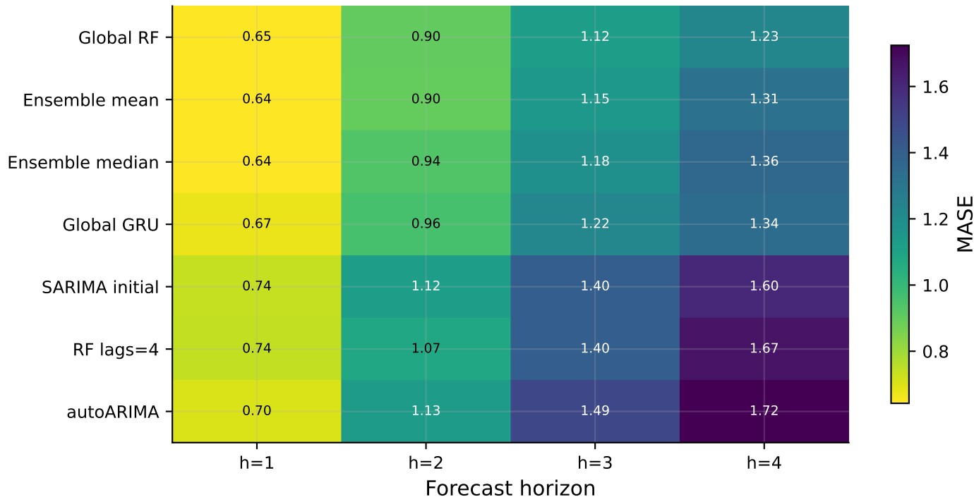
ILI - common6: MASE by model and horizon
