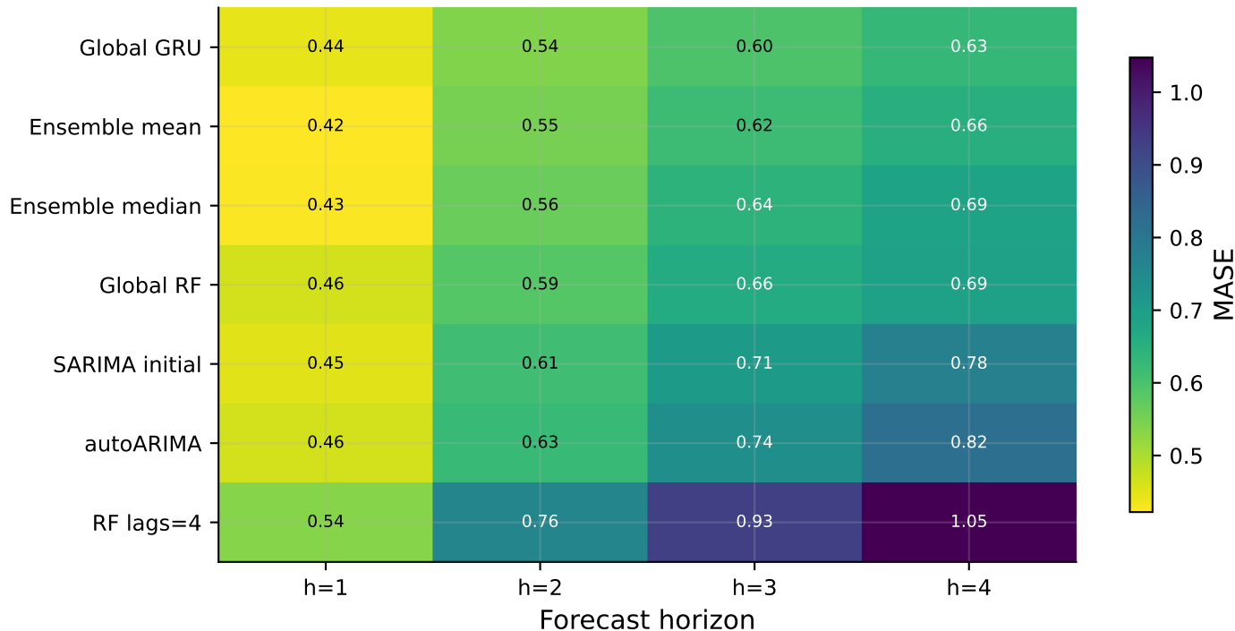
ARI - global: MASE by model and horizon
