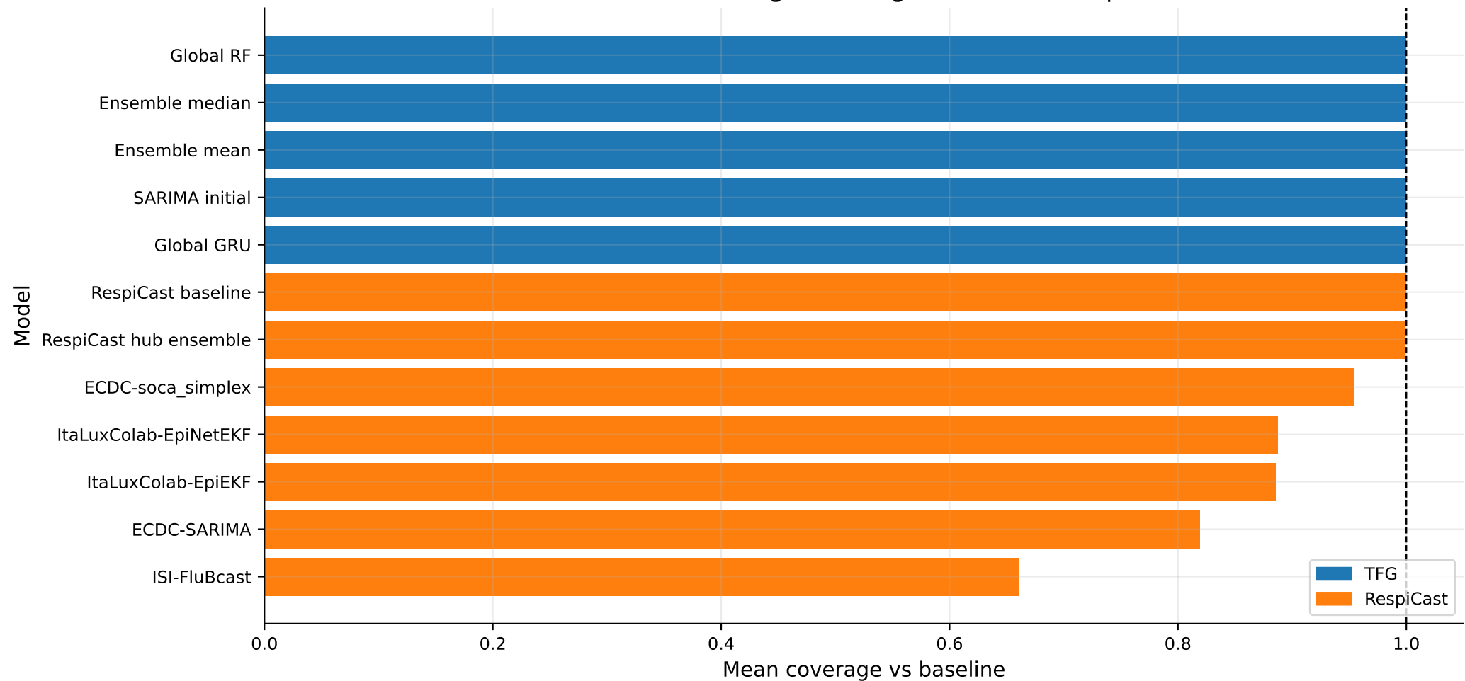
External benchmark: average coverage relative to RespiCast baseline
