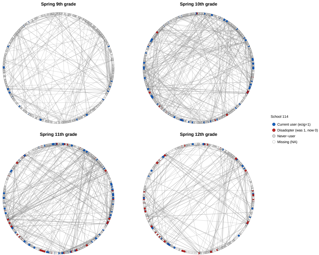
Figure 10: Figure 11.6.b — Same data, colour coding, and time slices as Figure 11.6.a, but with a community-ordered circular layout. Louvain community detection on the union graph yields 9 communities (sizes 62, 54, 50, 48, 44, 29, 27, 25, 19); these are arranged clockwise around the circle, largest first, and within each community nodes are ordered by degree (high \rightarrow low). The construction puts intra-community ties as short arcs near the perimeter and forces inter-community ties through the centre, making between-community contagion visible at a glance.
