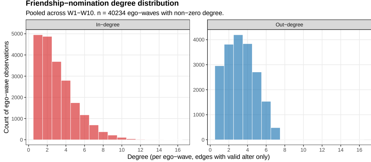
Figure 1: Out-degree and in-degree distributions across all valid (ego, wave) cells with non-zero degree.
