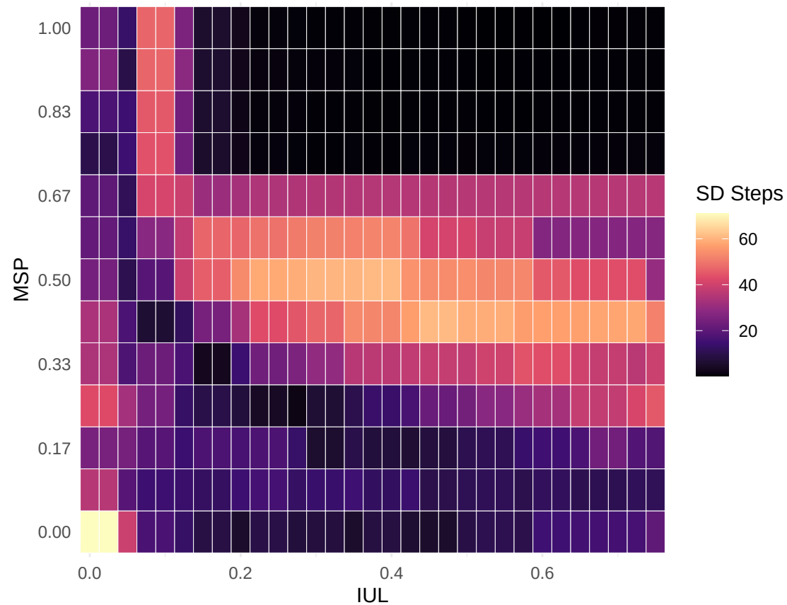
Method 2: Critical Slowing Down (SD of Steps)
