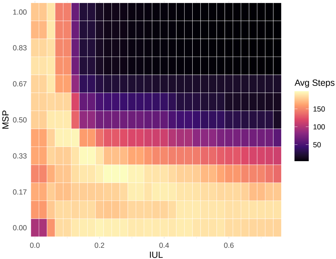
Method 2: Critical Slowing Down (Avg Steps)
