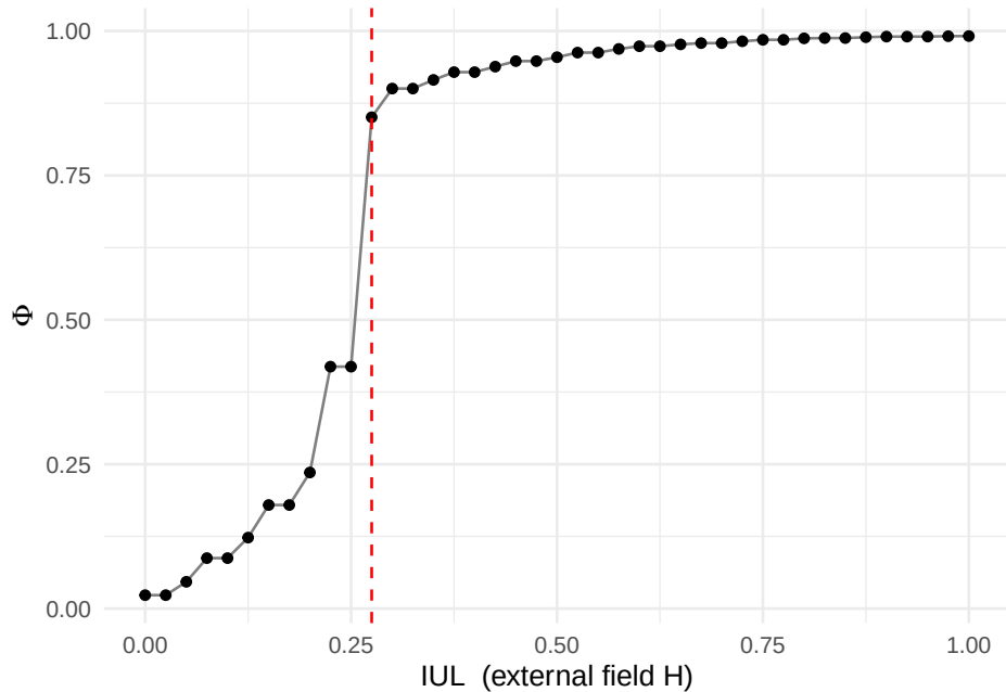
GSS: critical isotherm (MSP=0.25)
