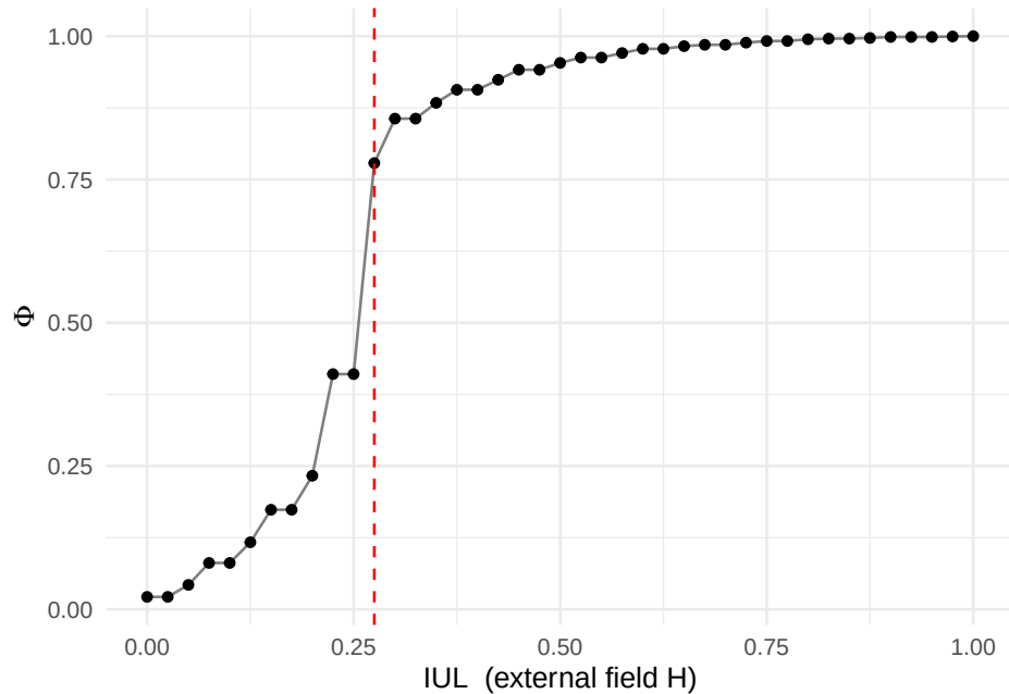
DP: critical isotherm (MSP=0.417)
