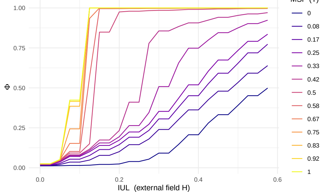
DP: isotherm family (Camino-H)
