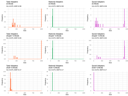
(a) GSS: Scale-free power-law bimodality.
