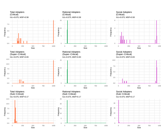
(a) GSS: Scale-free power-law bimodality.
