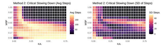
(b) Erdős-Rényi: Suppressed transition boundaries.
