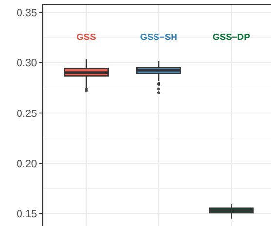
Modularity
