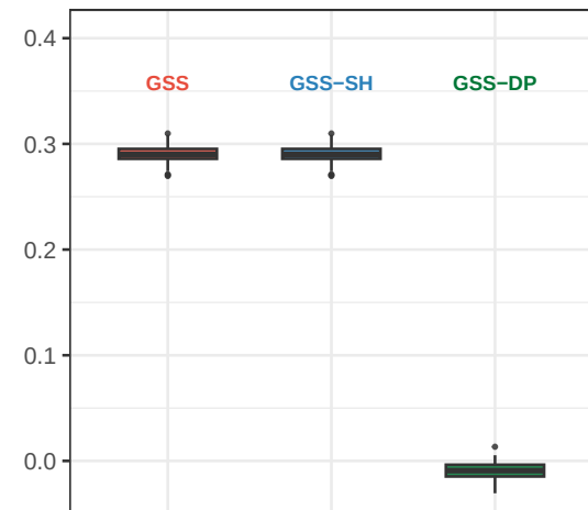
Degree assortativity
