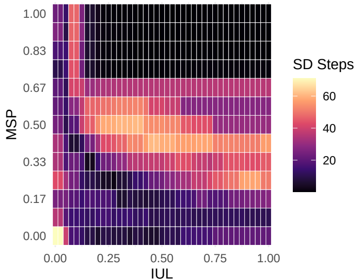
Method 2: Critical Slowing Down (SD of Steps)
