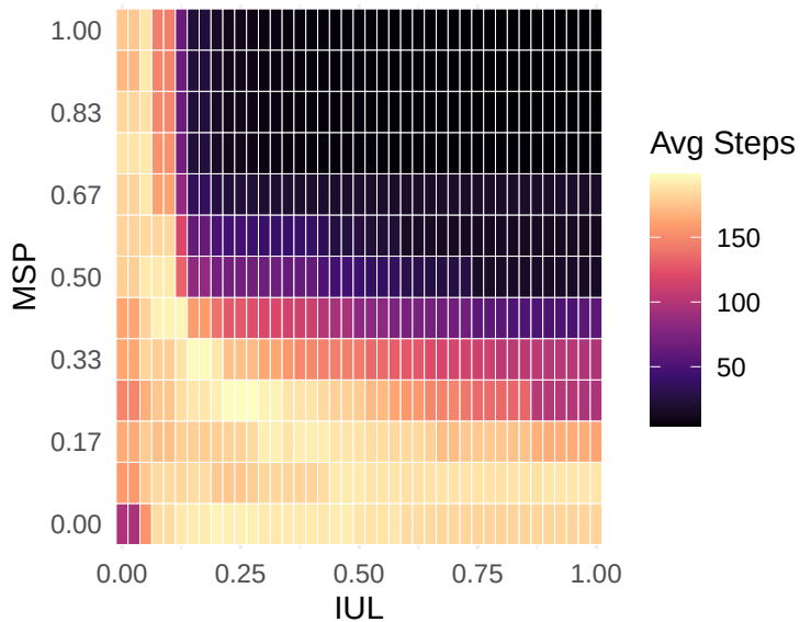
Method 2: Critical Slowing Down (Avg Steps)
