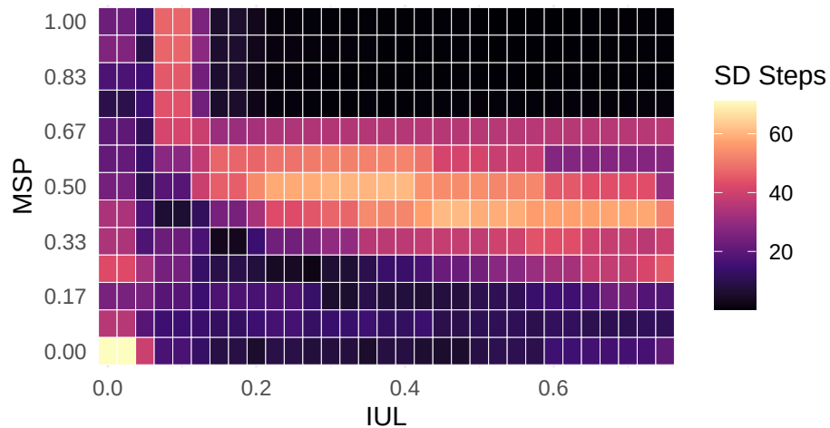
Method 2: Critical Slowing Down (SD of Steps)
