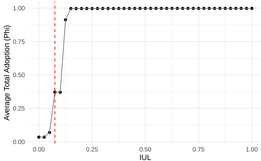
Method 4: Order Parameter (Phi) [MSP=0.50]
