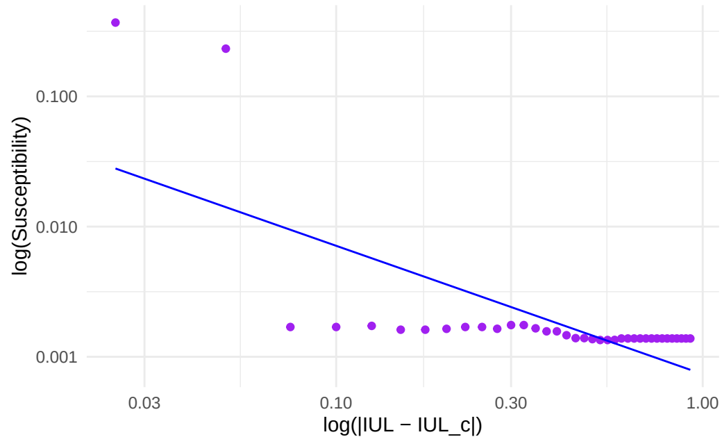
Method 4: Susceptibility Exponent
