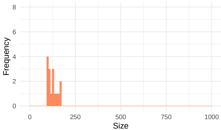
Total Adopters (Super-Critical) IUL=0.075, MSP=0.83
