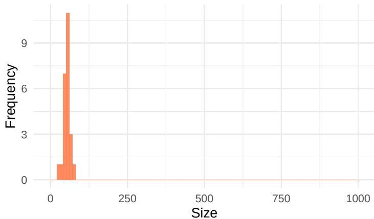
Total Adopters (Sub-Critical) IUL=0.075, MSP=0.17
