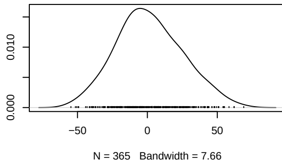
Density of gwesp.OTP.fixed.0.5
