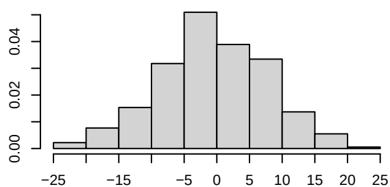
Density of nodematch.sexo
