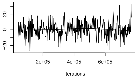
Trace of nodematch.disciplina
