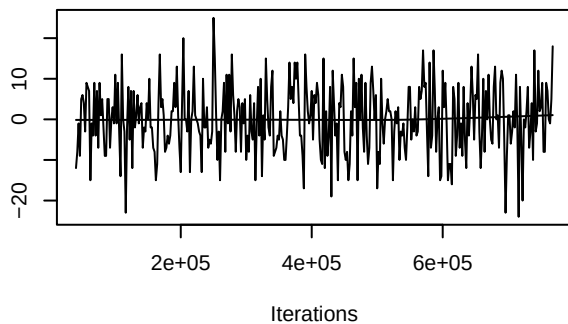
Trace of nodematch.sexo
