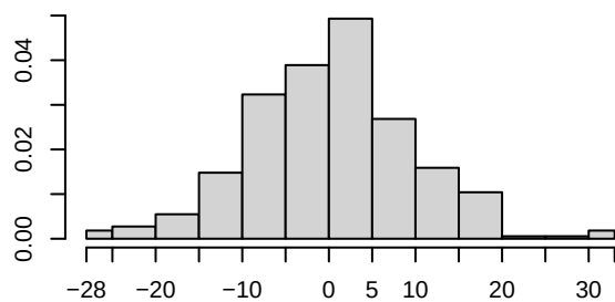
Density of nodematch.disciplina
