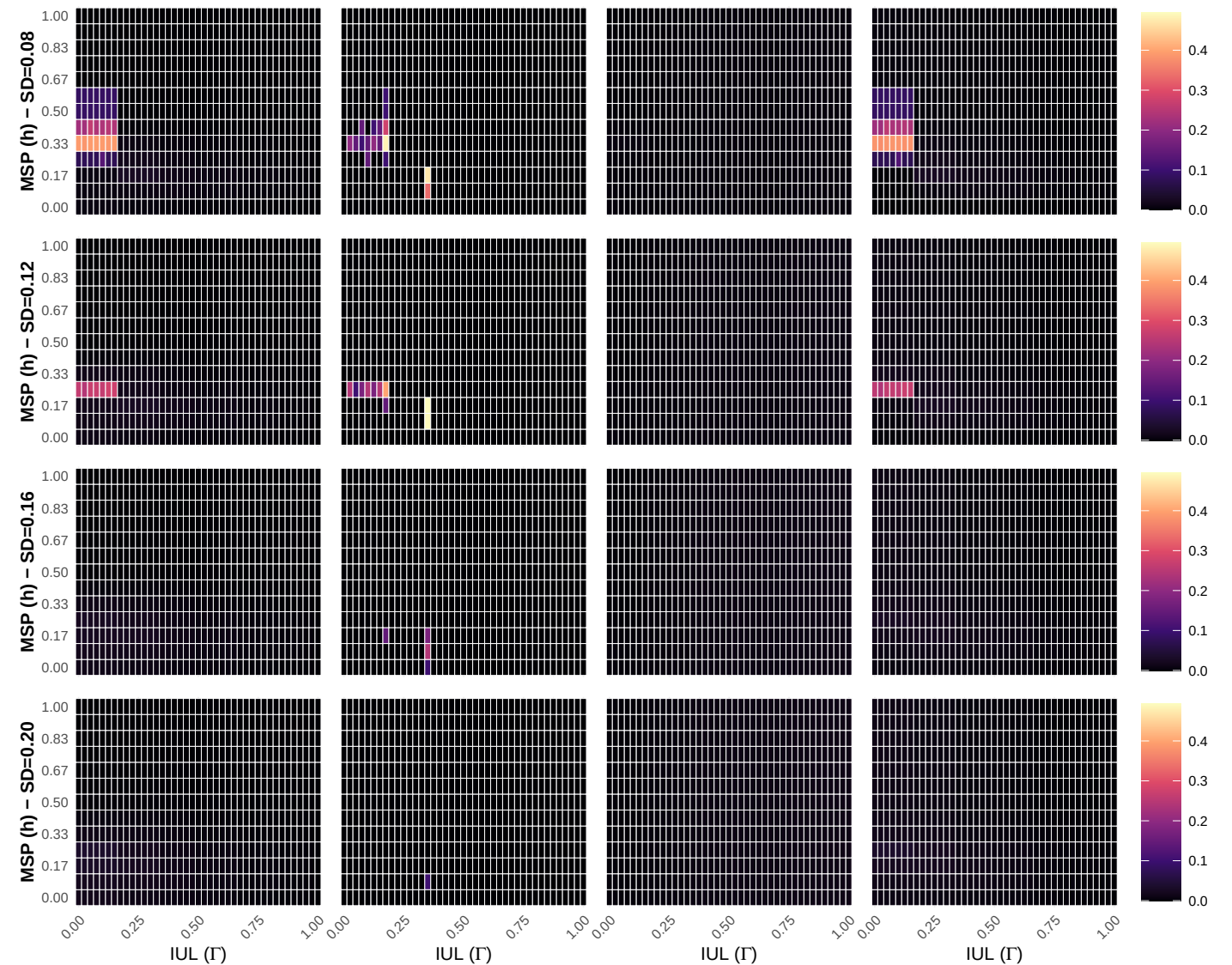
SD Adoption
