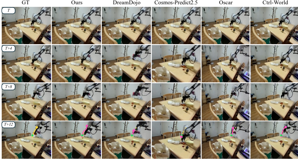
Figure 8: Tabletop scene. Columns: ground truth, SkeLAM, DreamDojo, Cosmos-Predict2.5, OSCAR, and Ctrl-World. Rows: T , T + 4 , T + 8 , and T + 12 . Colored markers and arrows highlight end-effector motion in the final row.
