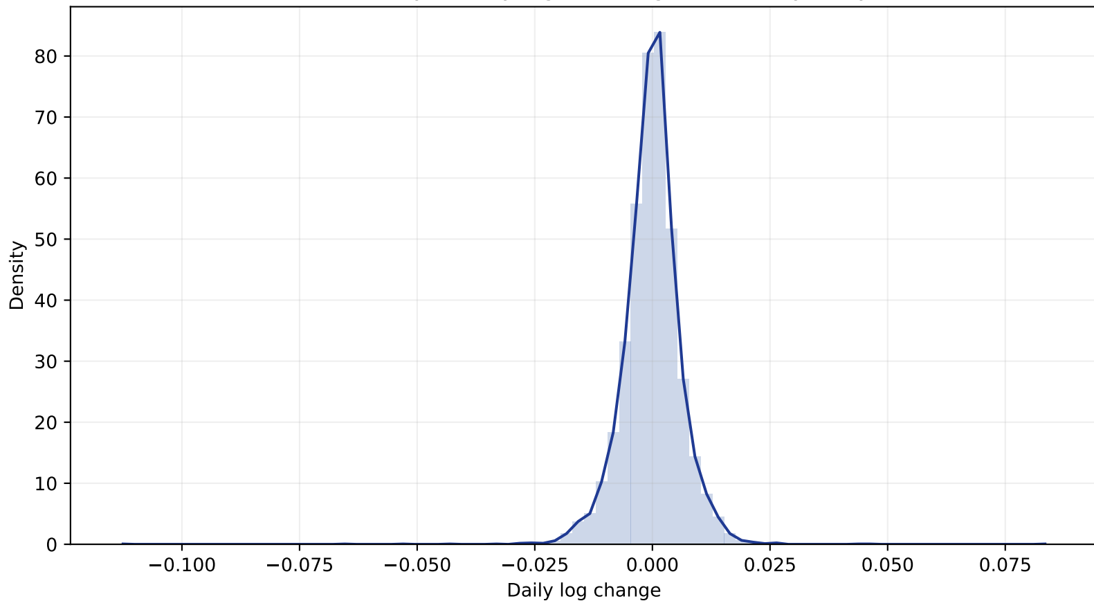
CHF: density of daily log FX changes (weekdays only)
