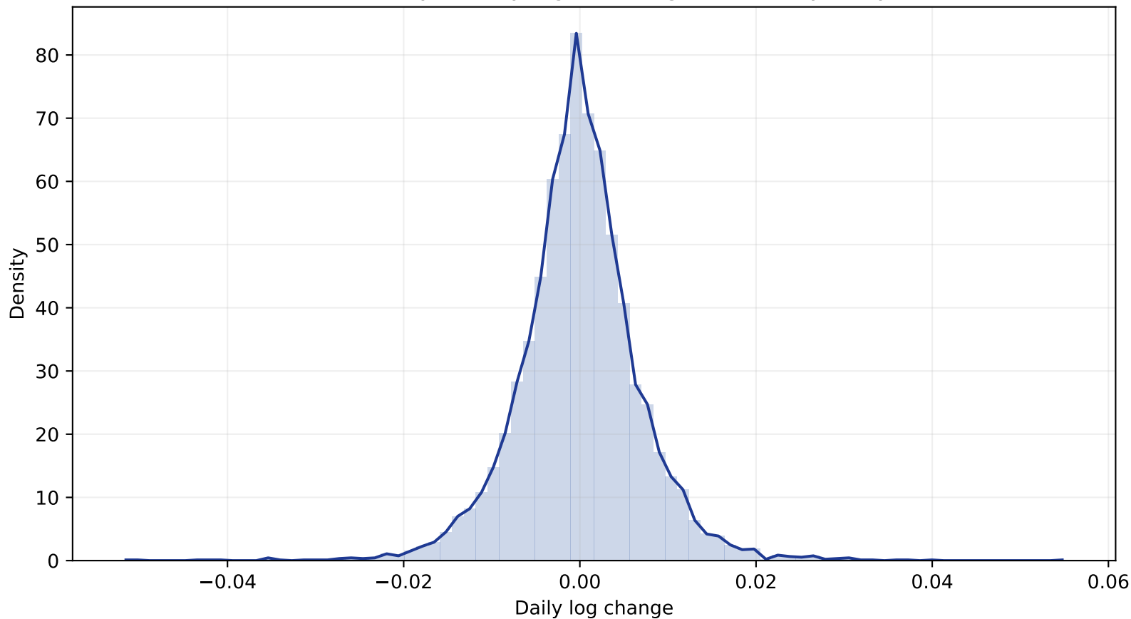
CZK: density of daily log FX changes (weekdays only)
