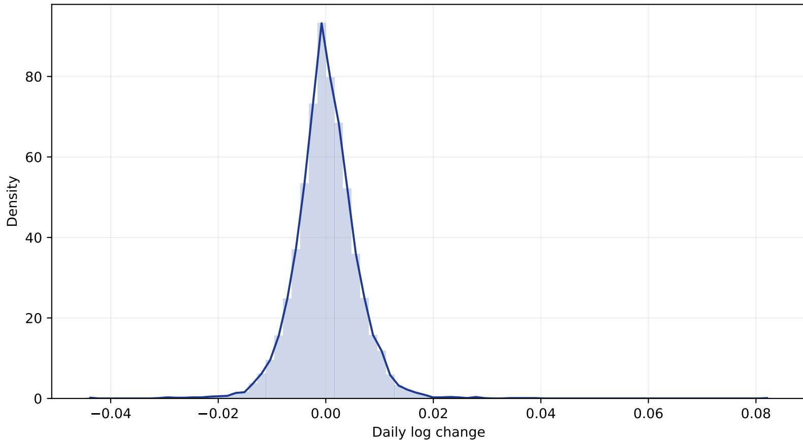
GBP: density of daily log FX changes (weekdays only)
