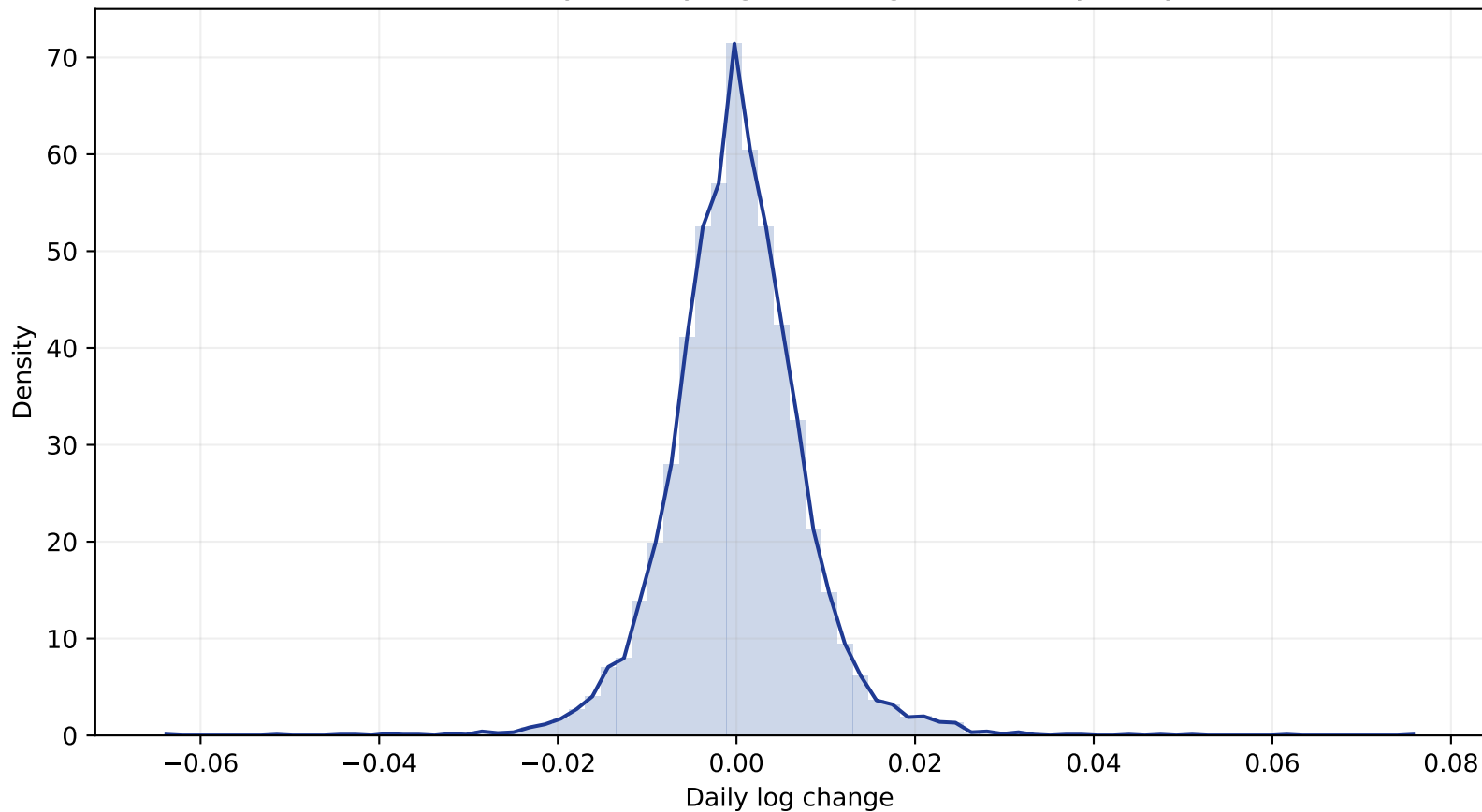
NOK: density of daily log FX changes (weekdays only)
