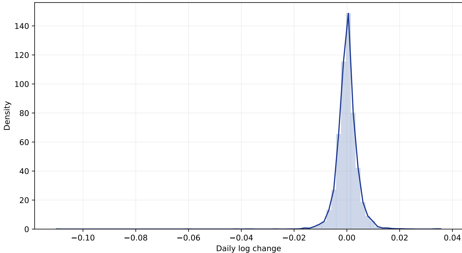
PHP: density of daily log FX changes (weekdays only)
