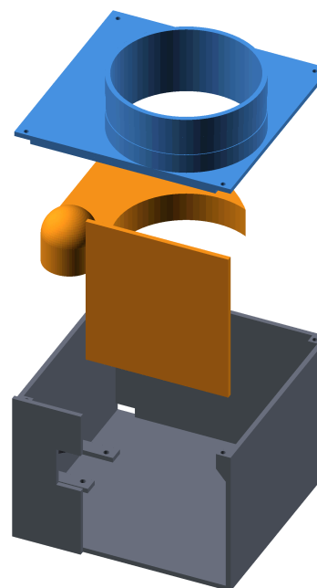
Printed Parts
