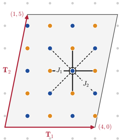
(b) tilted 20-site ( N=20 )
