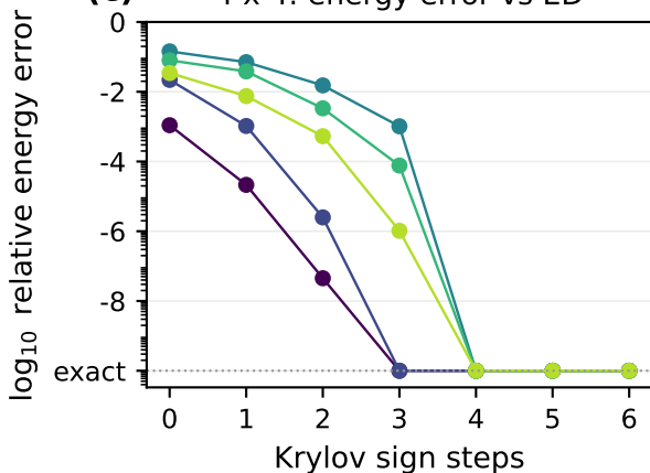
(c) 4 \times 4 : energy error vs ED
