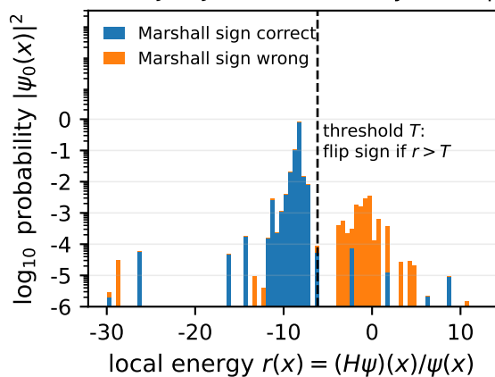
(a) 4 \times 4 , J_2 / J_1 = 0.5 : first Krylov step
