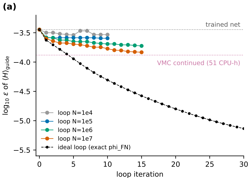
4x4 J1-J2 ( J_2/J_1=0.5 ): FN/Krylov loop started from a VMC-trained network (net H, 23.7k params)
