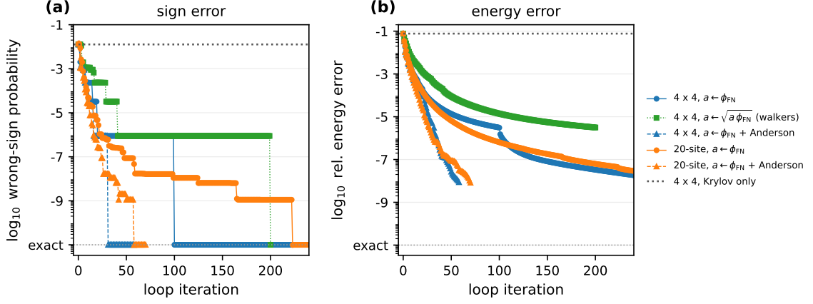
FIG. 5. Fixed-node-Krylov loop with exact diagonalization, started from the J_2 = 0 amplitude with Marshall signs, for three amplitude updates: a \leftarrow \phi_{\text{FN}} ; a \leftarrow \sqrt{a \phi_{\text{FN}}} , as learned from walkers; and a \leftarrow \phi_{\text{FN}} with Anderson extrapolation from the last three iterates. Dotted: Krylov steps alone from the same start, which change no sign. (a) Sign and (b) energy error vs iteration, compared with ED. All values are exact (no statistical error).
