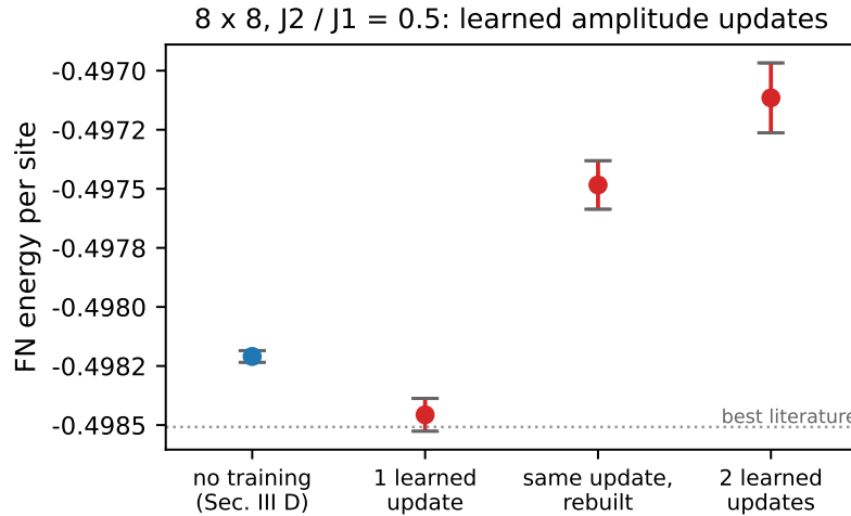
FIG. 10. 8 \times 8 fixed-node energy per site along learned amplitude updates (two walker populations each). Dotted: best same-geometry literature value [14].
